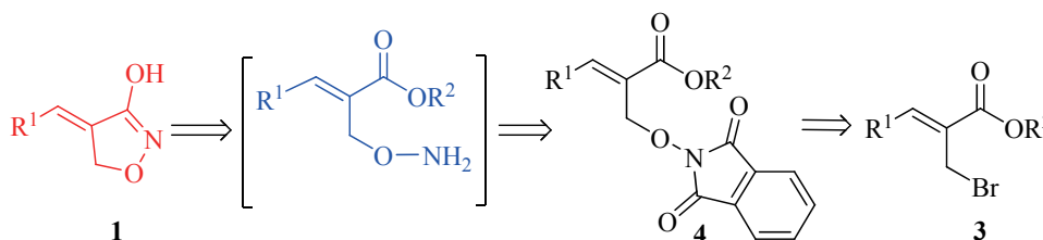
Scheme 1. Retrosynthetic approach for the synthesis of 4,5-dihydroisoxazol-3-ols
