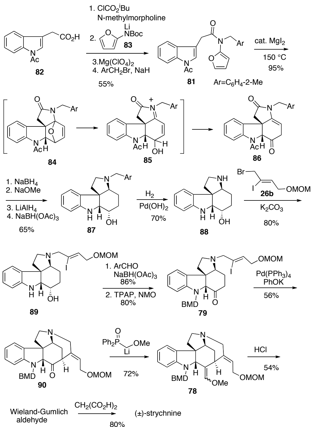
Scheme 17. Padwa's Total Synthesis of (±)-Strychnine
