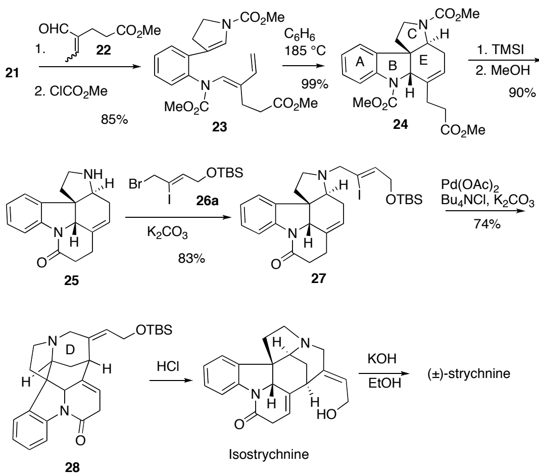
Scheme 4. Rawal's Total Synthesis of (\pm) -Strychnine
