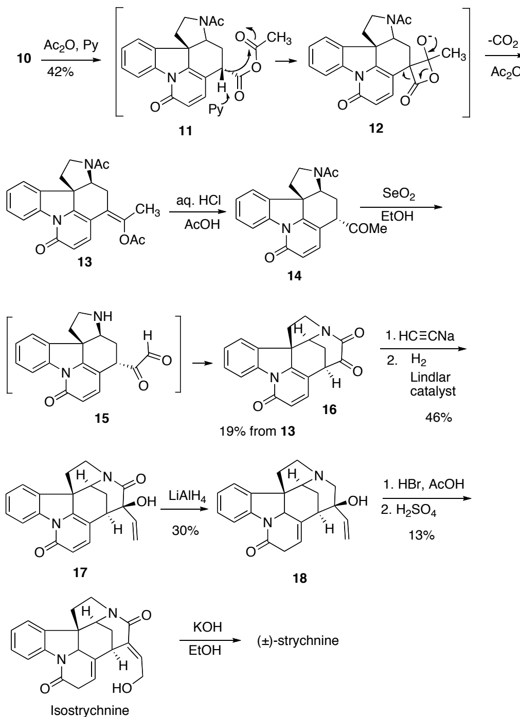
Scheme 2. Woodward's Total Synthesis of (±)-Strychnine
