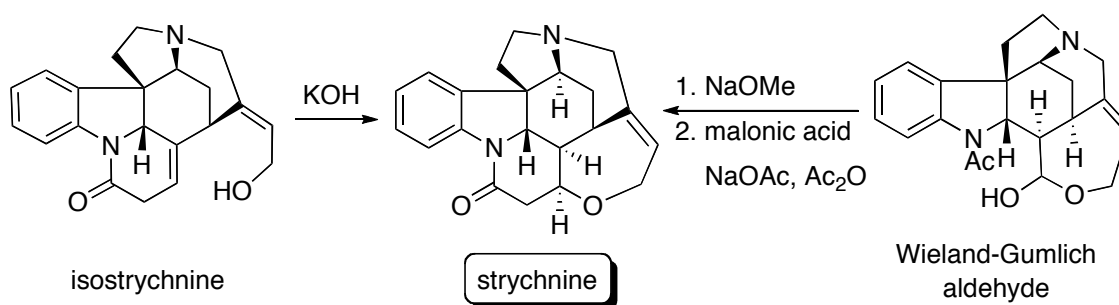
Scheme 5. Route to Synthesis of Strychnine
