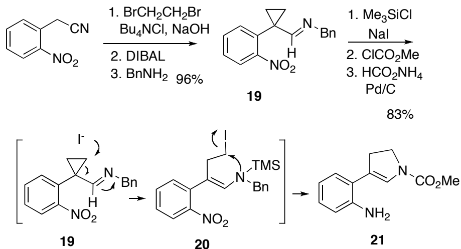
Scheme 3. Synthesis of Pyrroline 20 .
