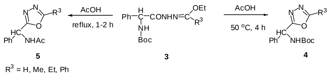
Scheme 5
