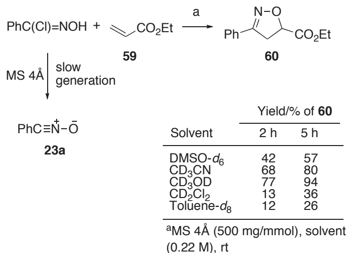
Scheme 5-49 Effect of the reaction solvent on the rate of generation of nitrile oxide 23a from benzohydroximoyl chloride
