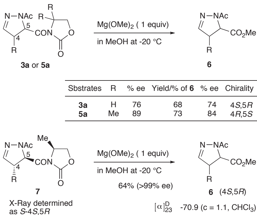
Scheme 4-02 Absolute configuration determination of 3a and 5a
