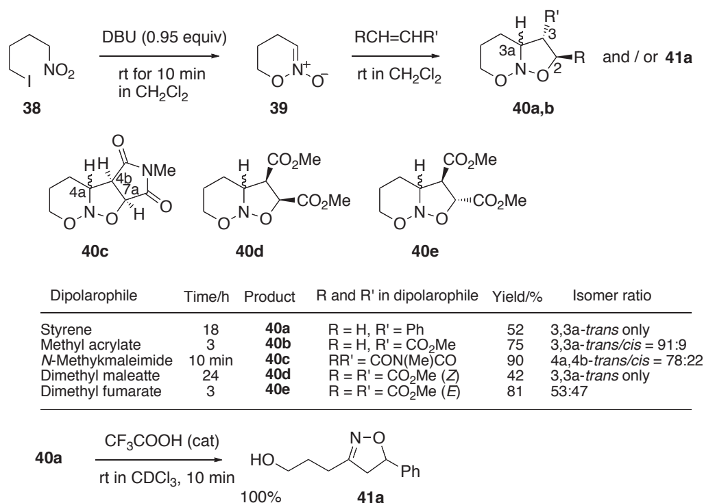
Scheme 3-11 Cycloaddition reactions of cyclic nitronate 39 with alkenes
