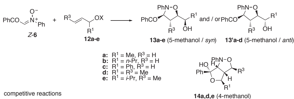
Scheme 3-04 1,3-Dipolar cycloadditions of benzoyl nitron 6 with \alpha -chiral allylic alcohols 12 in the presence of a catalytic amount of Lewis acid catalysts
