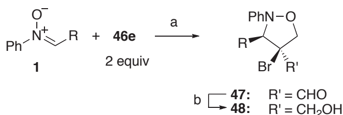
Scheme 3-20 Enantioselective nitron cycloaddition reactions to 2-bromoacrolein
