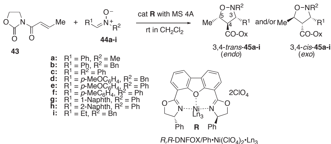
Scheme 3-13 Enantioselective cycloaddition reactions of nitrones 44a-i to 3-crotonoyl-2-oxazolidinone 43 under the catalysis of R,R -DBFOX/ Ph •Ni(ClO 4 ) 2 •Ln 3
