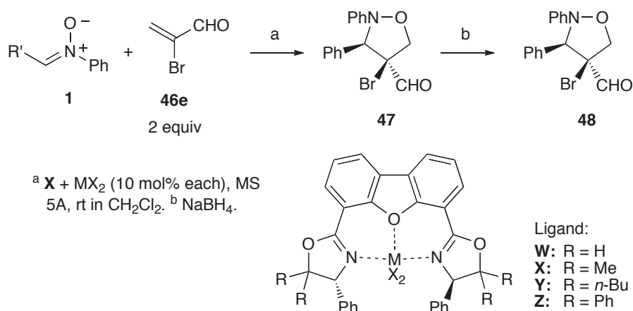
Scheme 3-22 Enantioselective cycloaddition reactions of nitrones 1 to 2-bromoacrolein 46e under the catalysis of R,R -tetramethylDBFOX/Ph complex X
