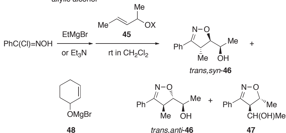
Scheme 5-35 Nitron cycloadditions to the magnesium alkoxide of inner and \alpha -chiral allylic alcohol
