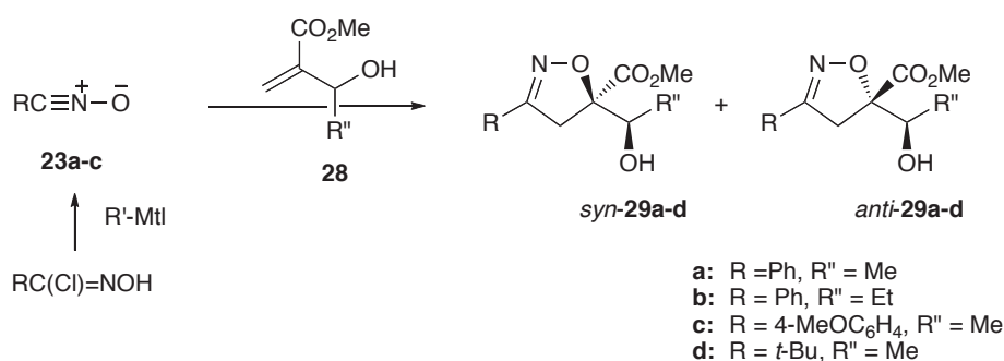
Scheme 5-16 Reactions of nitrile oxides 23a-c with methyl 2-(1-hydroxyalkyl)acrylate 28a,b
