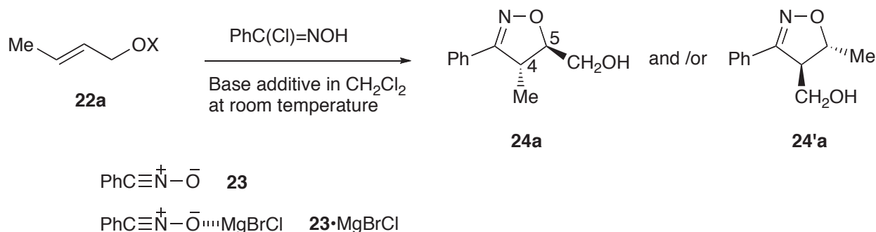
Scheme 5-09 Magnesium ion mediated regioselectivity control of nitrile oxide cycloadditions to ( E )-2-buten-1-ol 22a a
