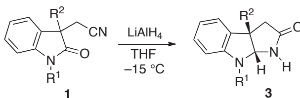
Scheme 3. \text{LiAlH}_4 -Reductive cyclization at low temperature
