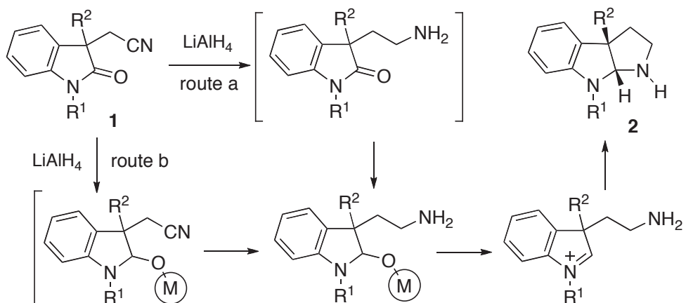
Scheme 2. Ambiguous routes of \text{LiAlH}_4 -reductive cyclization: M = Li or Al
