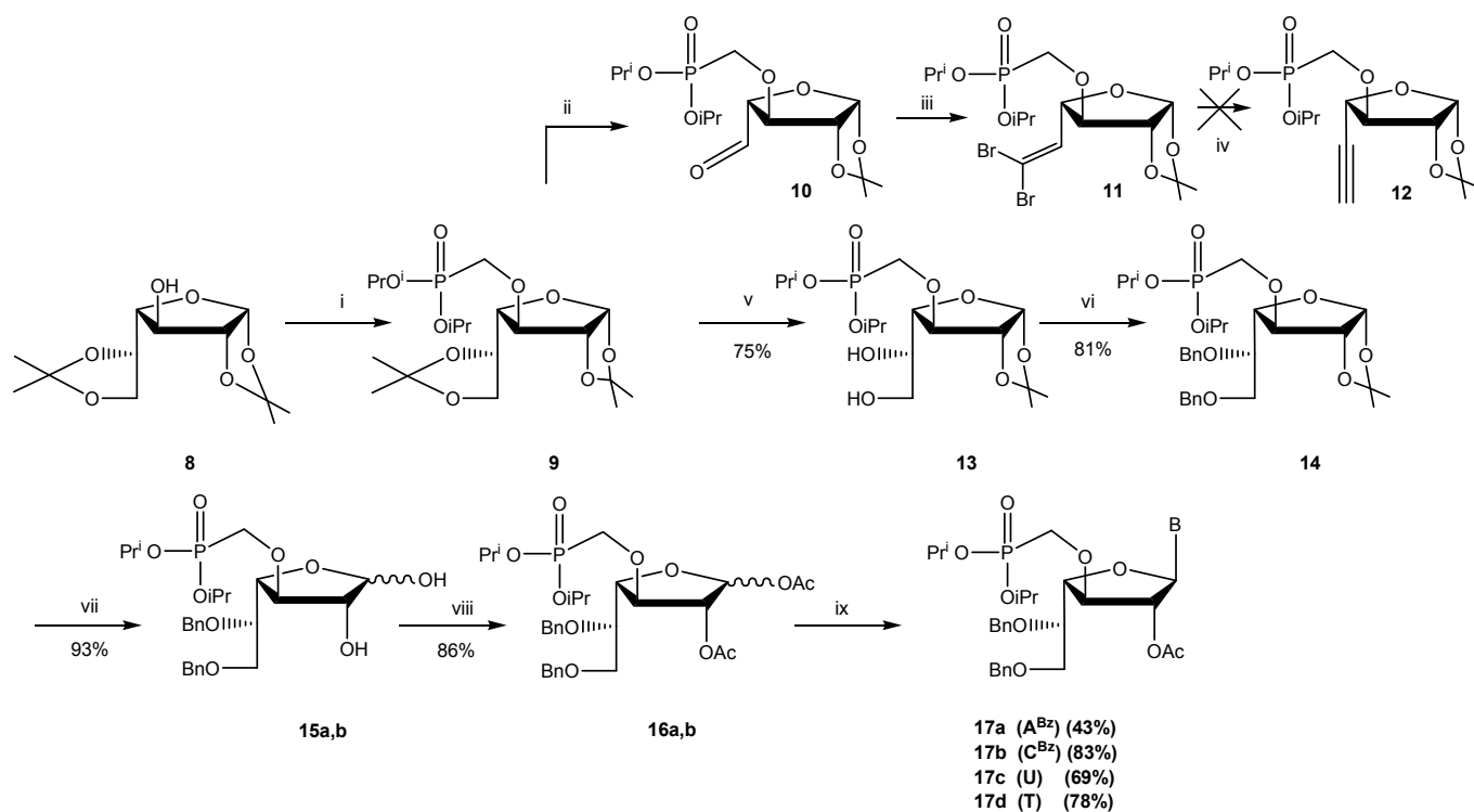
Scheme 1. i) NaH, THF, \text{P}(\text{O})(\text{OiPr})_2\text{CH}_2\text{OTf} , -78^\circ\text{C} , room temperature; ii) \text{H}_5\text{IO}_6 , \text{NaIO}_4 , \text{EtOAc} , room temperature; iii) \text{PPh}_3 , \text{CBr}_4 , \text{Et}_3\text{N} , \text{CH}_2\text{Cl}_2 ; room temperature iv) BuLi or MeONa; v) 70% AcOH, room temperature 20 h; vi) NaH, BnBr, DMF; vii) \text{CF}_3\text{CO}_2\text{H} , 1 h; viii) \text{Ac}_2\text{O} , pyridine, 0^\circ\text{C} ; ix) HMDS, (\text{NH}_4)_2\text{SO}_4 , \text{SnCl}_4 in \text{CH}_2\text{Cl}_2 , room temperature.
