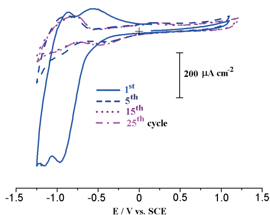
Figure 3. Cyclic voltammograms of B 12 -Ty ( 2 ) (1 mM) at a Pt electrode, (Pt-(P-Ty)/P(B 12 -Ty)), with a preformed polytyramine film in a 0.1 M LiClO 4 /CH 3 CN solution; v = 50 mV/s.
