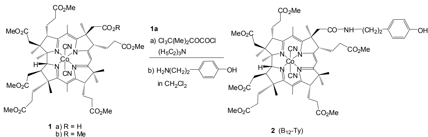
Scheme 1. Synthesis of Hexamethyl-cobyrinic Acid-c-Tyramide 'B 12 -Ty' (2).
