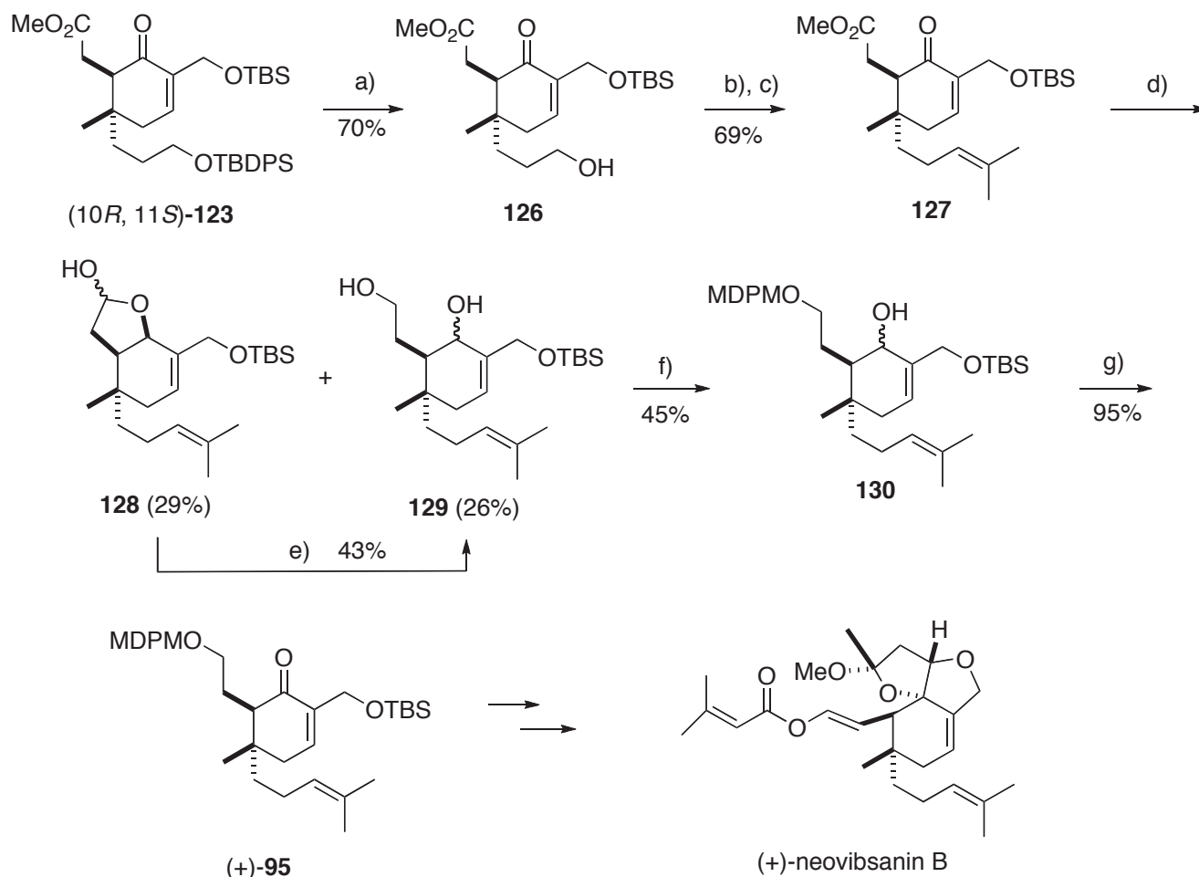
Scheme 13. Reagents and conditions: a) n -Bu 4 NF, AcOH, THF, rt; b) (COCl) 2 , DMSO, -78°C to 10°C, then Et 3 N; c) Me 2 CHP + Ph 3 I - , n -BuLi, THF, 0°C; d) DIBAL-H, CH 2 Cl 2 , -78°C; e) NaBH 4 , EtOH, rt; f) 2,4-DMPM-trichloroacetoimide, 10 mol% CSA, CH 2 Cl 2 , -20°C; g) Dess-Martin periodinane, CH 2 Cl 2 , rt.
