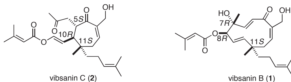
Figure 5. Absolute configurations of vibsanins B ( 1 ) and C ( 2 )
