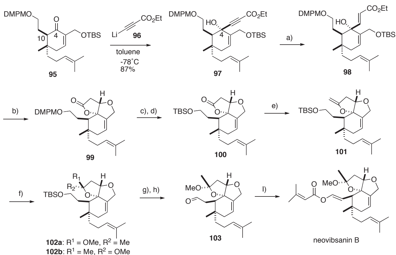
Scheme 10. Reagents and conditions: a) Red-Al, THF, -78^\circ\text{C} , 87%; b) TBAF, THF, rt, 87%; c) DDQ, \text{CH}_2\text{Cl}_2 /phosphate buffer, NaCl, 0^\circ\text{C} , 83%; d) TBSCl, imidazole, 0^\circ\text{C} to rt, 99%; e) Tebbe reagent, pyridine, THF-toluene; f) PPTS, MeOH, 0^\circ\text{C} , 91%; g) TBAF, THF, rt, 99%; h) \text{SO}_3 /pyridine, \text{Et}_3\text{N} , DMSO, rt, 89%; i) KHMDS, THF, then 3,3-dimethylacryloyl chloride, -78^\circ\text{C} , 60%.
