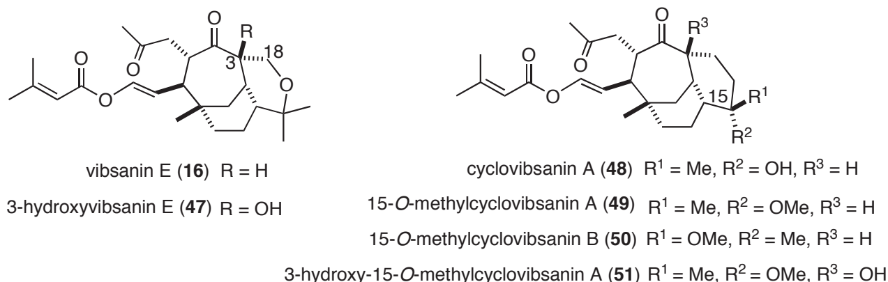
Figure 10. 7-Membered ring tricyclic vibsanins
