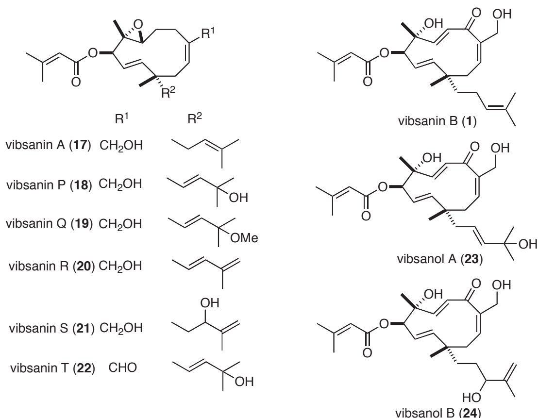
Figure 8. 11-Membered ring vibsanins
