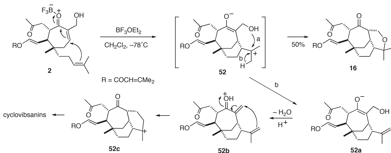
Scheme 5. Conversion of vibsanin C ( 2 ) to vibsanin E ( 16 ) and a plausible biosynthetic pathway for cyclovibsanins
