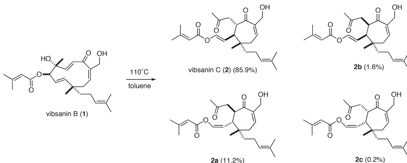
Scheme 1. Oxy -Cope rearrangement of vibsanin B ( 1 )
