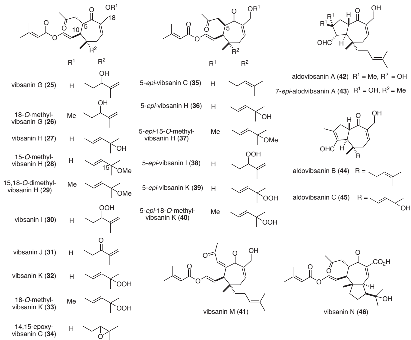
Figure 9. 7-Membered ring vibsananins
