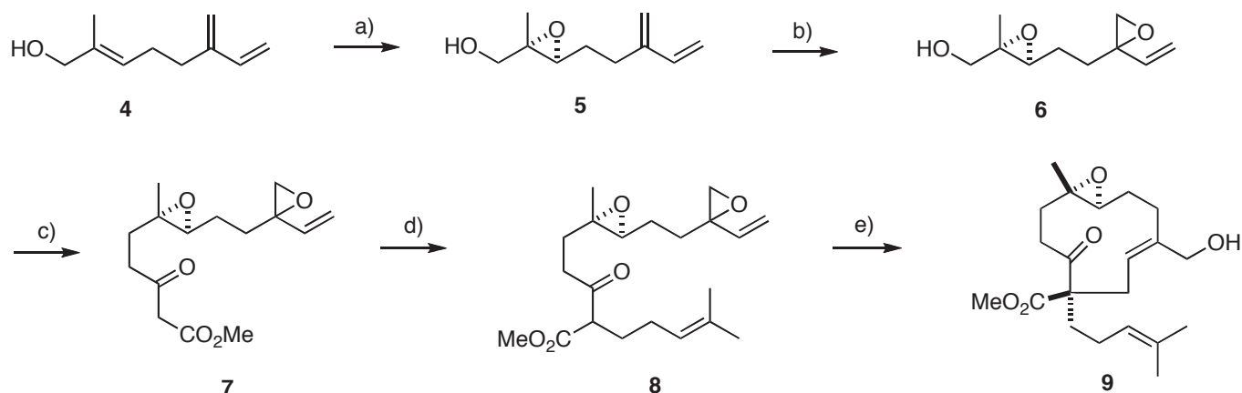
Scheme 3. Reagents and conditions: a) \text{Ti}(\text{OiPr})_4 , L-(+)-DET, TBHP, MS4A, \text{CH}_2\text{Cl}_2 , -35^\circ\text{C} , 99% (92% ee); b) MCPBA, \text{CH}_2\text{Cl}_2 , 0^\circ\text{C} , 91%; c) \text{Tf}_2\text{O} , \text{Et}_3\text{N} , THF, -78^\circ\text{C} , then 5 eq. the dianion of methyl acetoacetate generated with NaH and n\text{BuLi} , THF, 0^\circ\text{C} , 94%; d) NaH, 15-crown-5, DMSO, then 5-iodo-2-methylpent-2-ene, 77%; e) 10 mol% \text{Pd}(\text{PPh}_3)_4 , DMSO, 90^\circ\text{C} , 60%.
