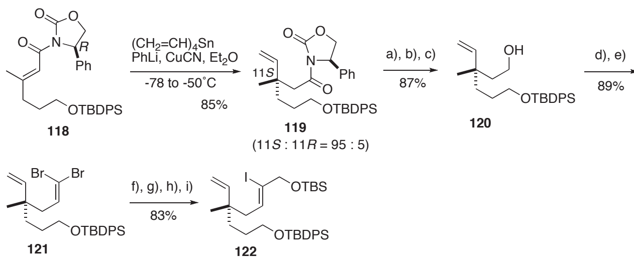
Scheme 12. Reagents and conditions: a) 30% \text{H}_2\text{O}_2 , \text{LiOH} , \text{THF-H}_2\text{O} , 0^\circ\text{C} ; b) \text{EtOH} , \text{EDC} , \text{DMAP} , \text{CH}_2\text{Cl}_2 , \text{rt} ; c) \text{LiAlH}_4 , \text{THF} , 0^\circ\text{C} ; d) \text{PCC} , celite, \text{CH}_2\text{Cl}_2 , 0^\circ\text{C} ; e) \text{CBr}_4 , \text{PPh}_3 , \text{CH}_2\text{Cl}_2 , 0^\circ\text{C} ; f) n\text{-BuLi} , \text{THF} , -78^\circ\text{C} , then (\text{CH}_2\text{O})_n , \text{rt} ; g) \text{Bu}_3\text{SnH} , \text{AIBN} , \text{THF} , reflux; h) \text{I}_2 , \text{CH}_2\text{Cl}_2 , 0^\circ\text{C} ; i) \text{TBSCl} , \text{DMAP} , \text{Et}_3\text{N} , \text{CH}_2\text{Cl}_2 , \text{rt} .
