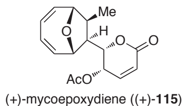
Figure 7. Structure of (+)-mycoepoxydiene ((+)- 115 )
