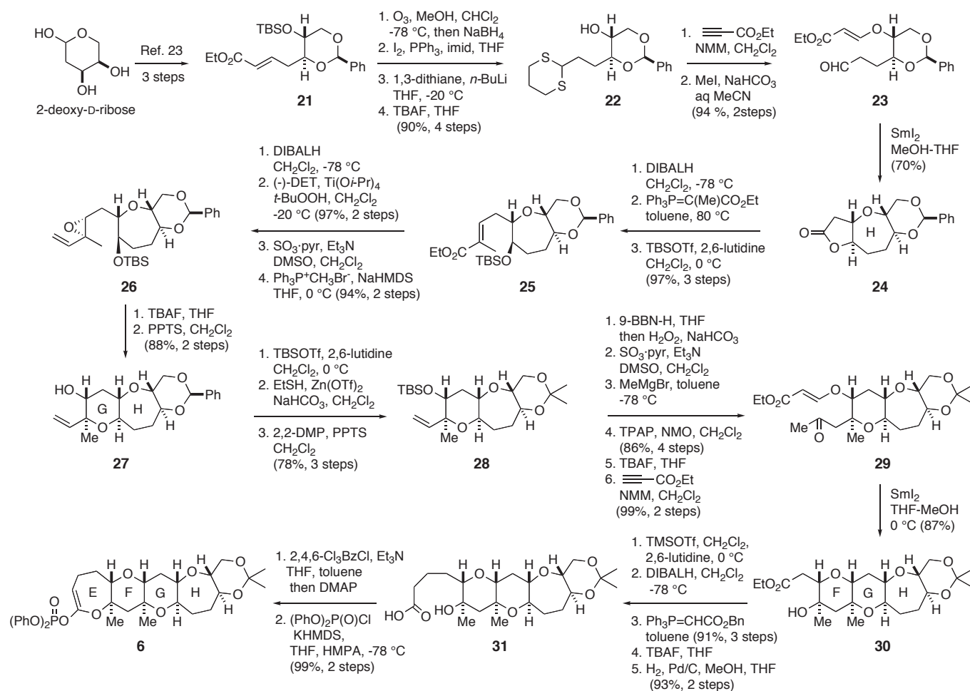
Scheme 4. Sasaki's synthesis of the EFGH-ring fragment 6
