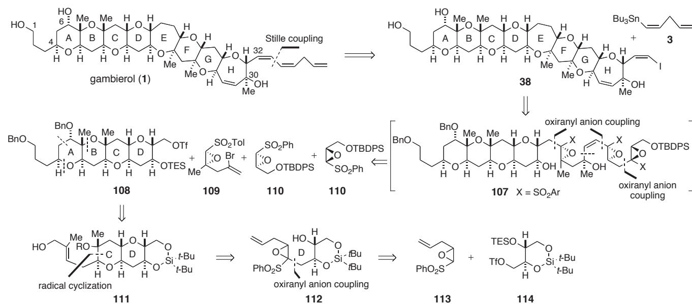
Scheme 17. Mori's retrosynthesis of gambierol
