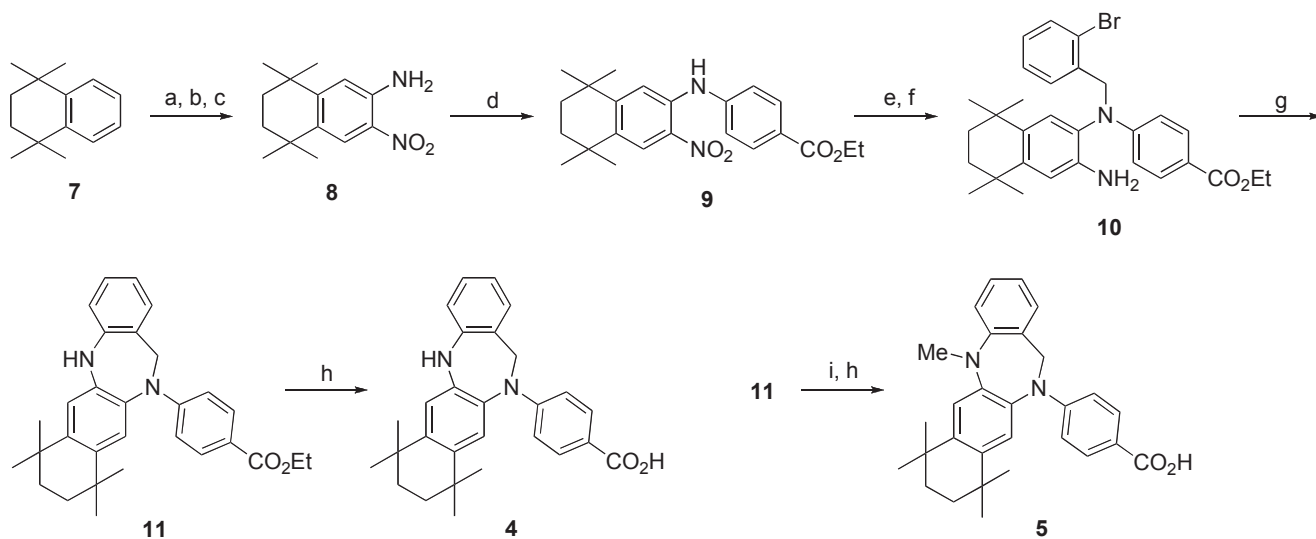
Scheme 1. Synthesis of dibenzodiazepine derivatives 4 and 5 ; Reagents and conditions: (a) c.H 2 SO 4 , HNO 3 , AcOH, rt, 44%; (b) Pd/C, H 2 , EtOH, rt, 94%; (c) c.H 2 SO 4 , HNO 3 , TFA, rt, 38%; (d) Pd 2 (dba) 3 , rac -BINAP, NaO t Bu, ethyl 4-iodobenzoate, toluene, reflux, 34%; (e) NaH, o -bromobenzyl bromide, DMF, rt, 98%; (f) Zn, AcOH, rt, 43%; (g) Pd 2 (dba) 3 , rac -BINAP, NaO t Bu, toluene, reflux, 100%; (h) 20% KOH aq., EtOH, rt, quant; (i) NaH, MeI, DMF, rt, quant.
