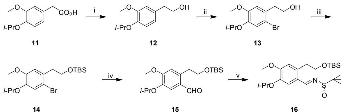
Scheme 2. Reagents and conditions: (i) \text{LiAlH}_4 , THF, reflux 2 h, 98%; (ii) NBS, DMF, rt, 12 h, 98%; (iii) TBSCl, imidazole, \text{CH}_2\text{Cl}_2 , rt, 91%; (iv) n\text{-BuLi} , THF, DMF, -78 \sim 0^\circ\text{C} , 93%; (v) ( S )- tert -butanesulfinamide, \text{Ti}(\text{O}i\text{-Pr})_4 , THF, reflux 4 h, 92%.
