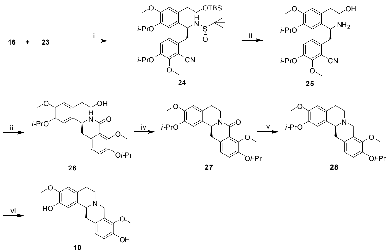
Scheme 4. Reagents and conditions: (i) LDA, THF, -78 °C, 52%; (ii) MeOH, conc. HCl, rt, 81%; (iii) KOH, H 2 O-EtOH, reflux 20 h, 87%; (iv) TsCl, pyridine, rt, 8 h; NaH, THF, 0 °C, 2 h. 67% for 2 steps; (v) LiAlH 4 , THF, reflux 2 h, 91%; (vi) BCl 3 , CH 2 Cl 2 , -78 °C, 82%.
