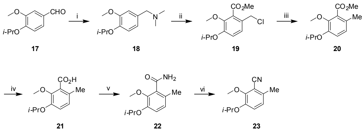
Scheme 3. Reagents and conditions: (i) a. \text{Me}_2\text{NH}\cdot\text{HCl} , \text{Et}_3\text{N} , \text{Ti}(\text{O}i\text{-Pr})_4 , EtOH, rt, 12 h; b. \text{NaBH}_4 , 8 h, 82%; (ii) n\text{-BuLi} , THF, \text{ClCO}_2\text{Me} , -78 \sim 0^\circ\text{C} , 93%; (iii) \text{H}_2 , Pd/C, MeOH, 4 h, 97%; (iv) NaOH, \text{H}_2\text{O} -EtOH, reflux 2 h, 96%; (v) a. (\text{COCl})_2 , reflux 2 h; b. \text{NH}_4\text{OH} , 88%; (vi) cyanuric chloride, DMF, rt, 16 h, 95%.
