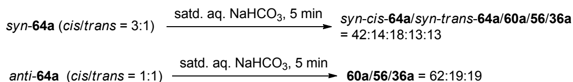
Scheme 24. Synthesis of sulfonium salts 64 and reactions with NaHCO 3
