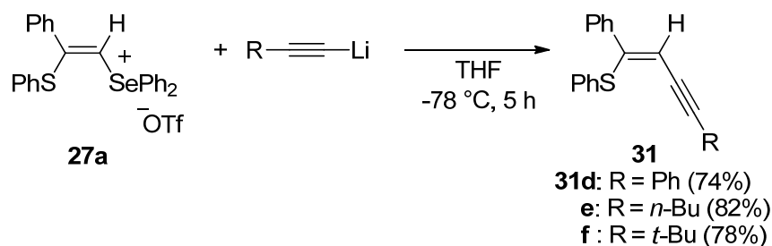
Scheme 15. Reaction of ( Z )-β-phenylthiovinylselenonium salt with acetylide
