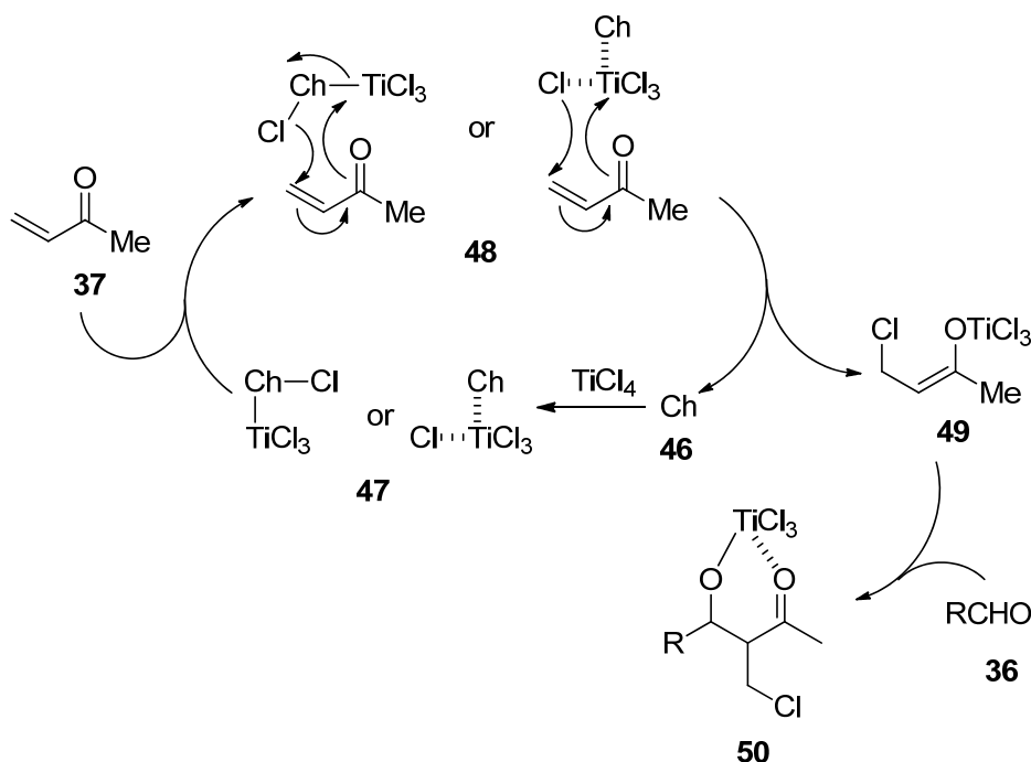
Scheme 20. Mechanism for the formation of \alpha -chloromethyl aldols
