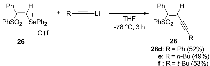
Scheme 12. Reaction of (Z)-β-phenylsulfonylvinylselenonium salt with acetylenes
