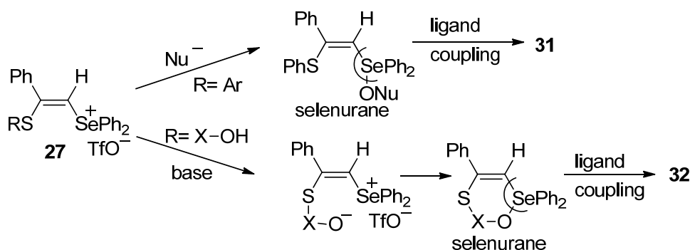
Scheme 16. Plausible mechanism for the reaction of ( Z )-β-thiovinylselenonium salts with nucleophiles
