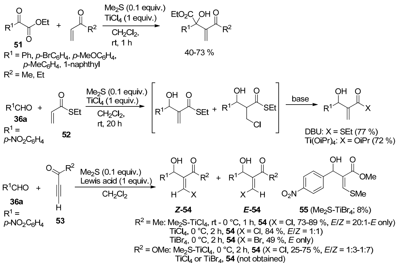
Scheme 21. Various tandem Michael-aldol reactions mediated by chalcogenide-TiCl 4
