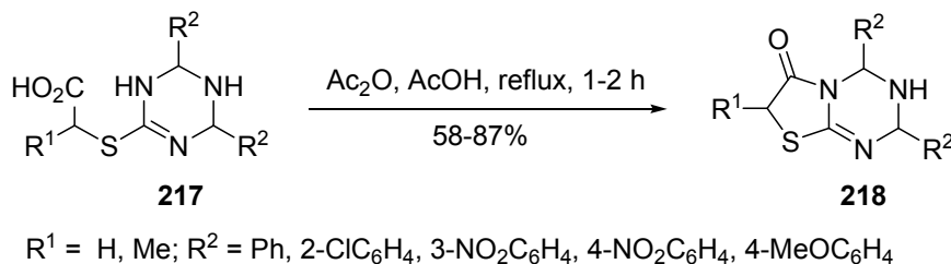
Scheme 99
