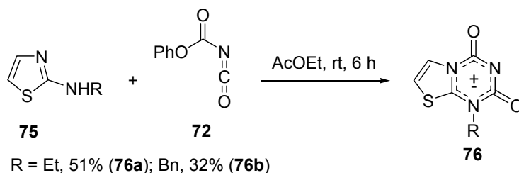
Scheme 33
