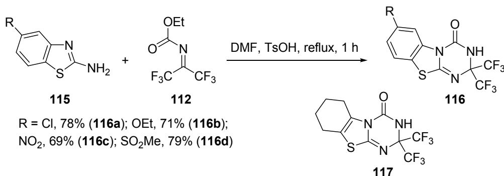
Scheme 48
