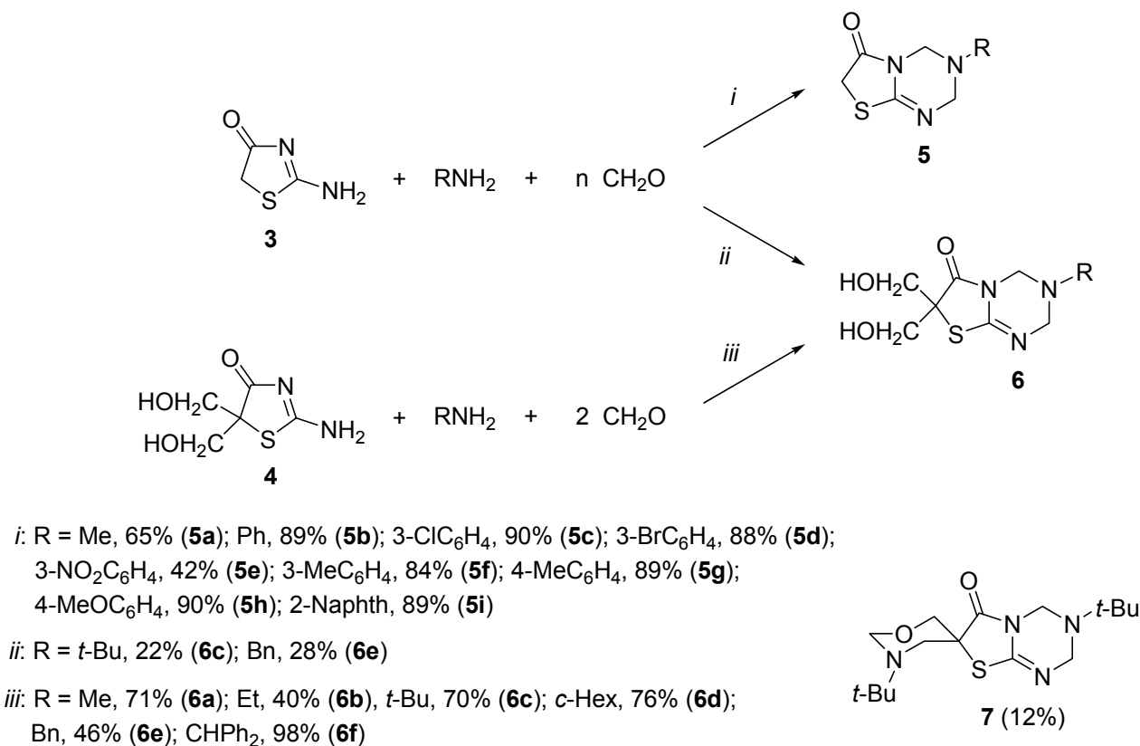
Scheme 2
