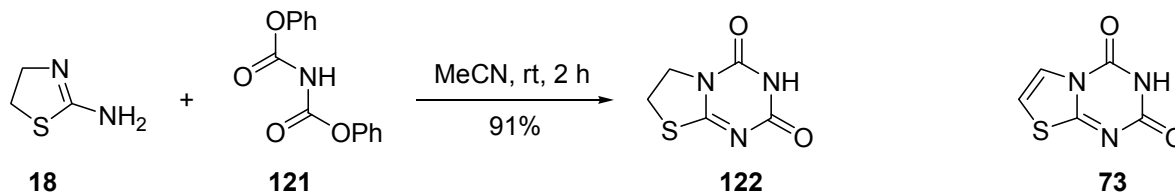
Scheme 50
