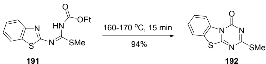
Scheme 86
