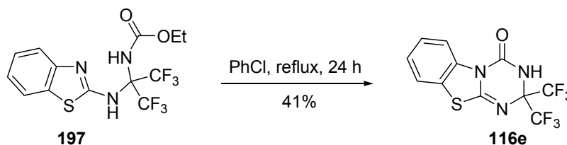
Scheme 90
