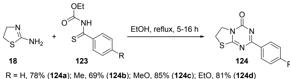
Scheme 51
