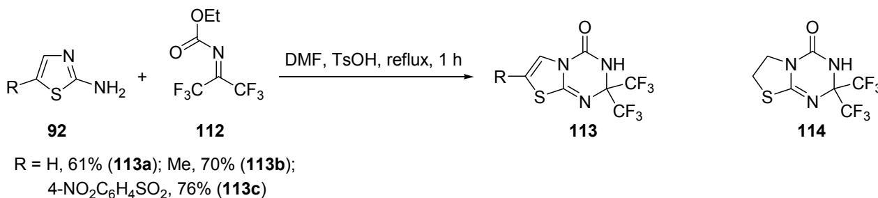
Scheme 47
