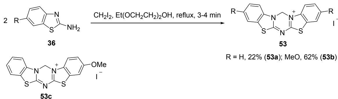
Scheme 23
