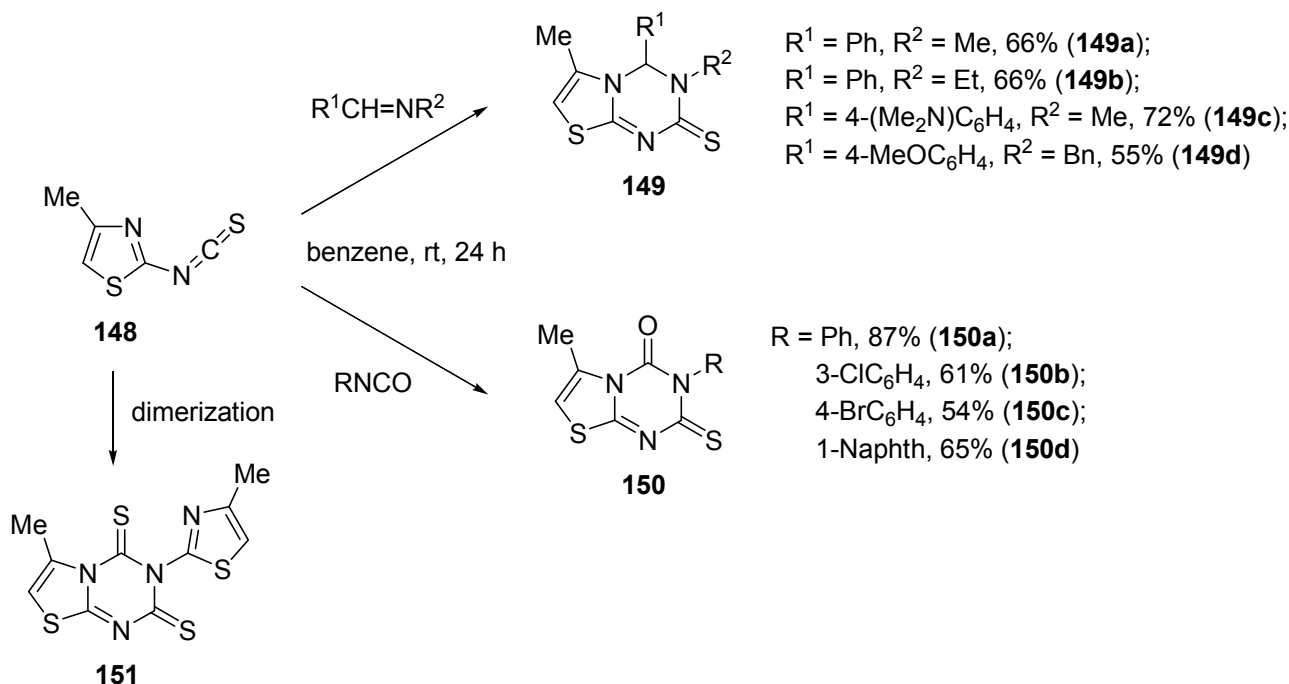
Scheme 63
