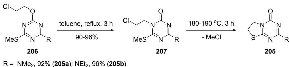
Scheme 95
