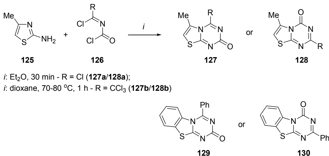
Scheme 52
