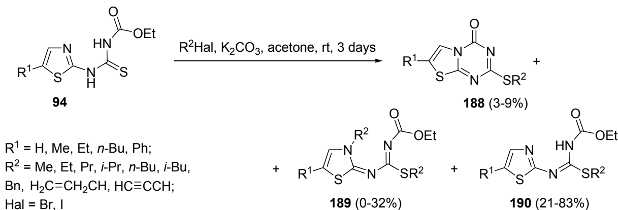
Scheme 84
