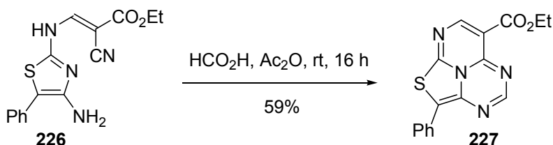
Scheme 103
