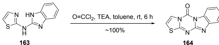
Scheme 71
