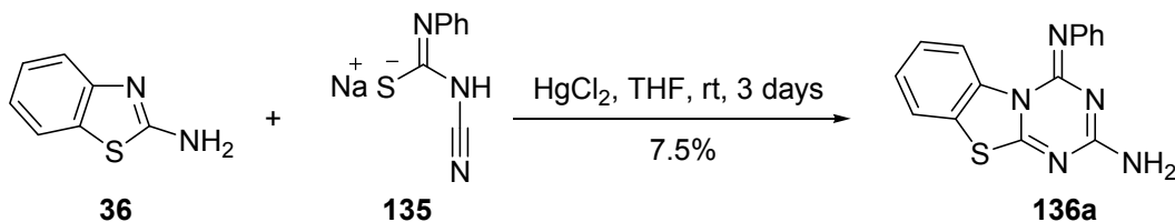
Scheme 55
