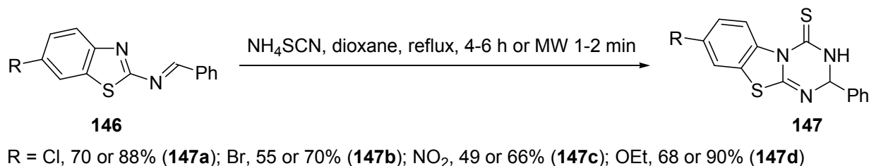
Scheme 62
