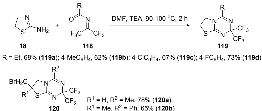
Scheme 49
