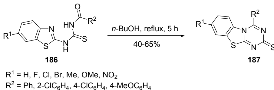
Scheme 82
