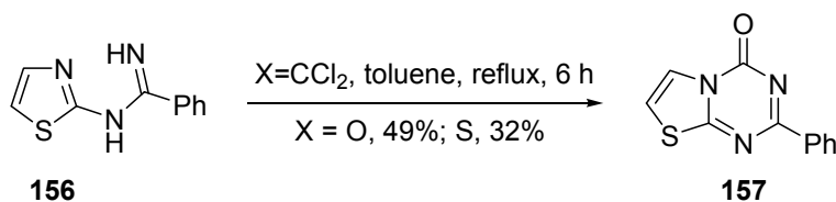
Scheme 67
