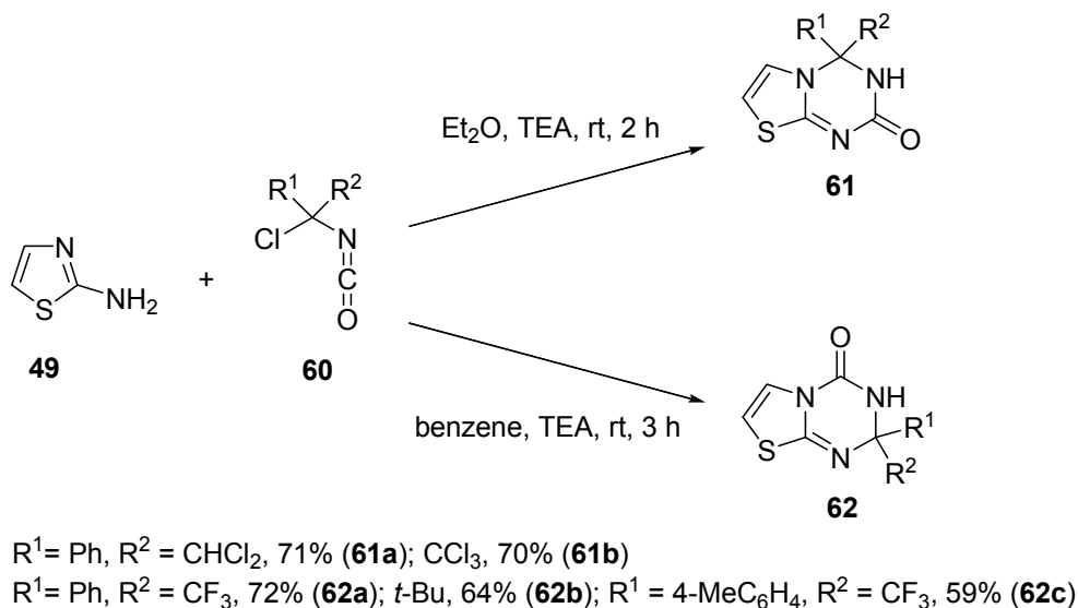
Scheme 27
