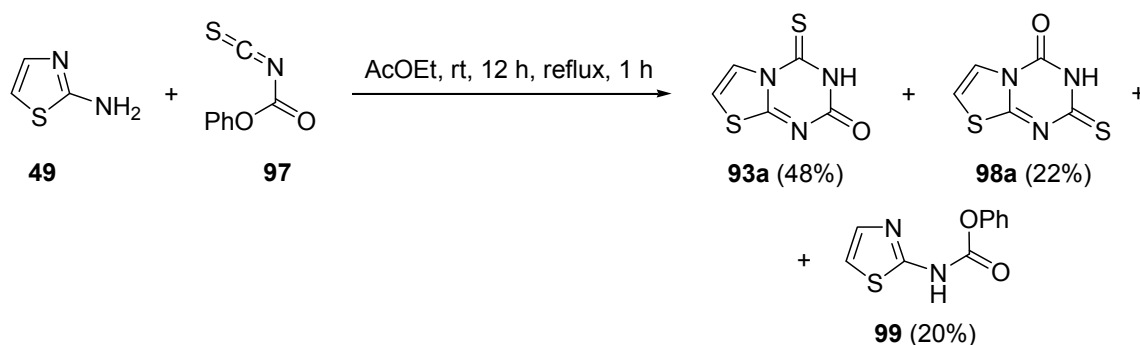
Scheme 42
