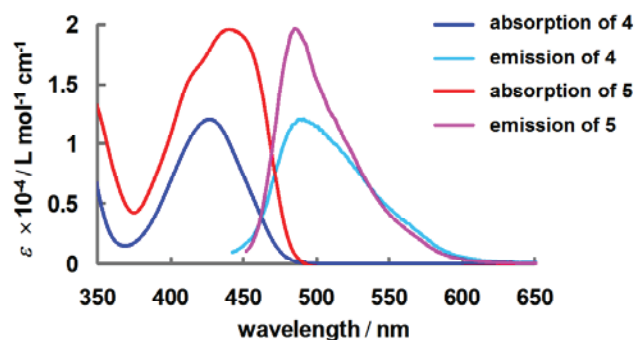
Figure 2. UV-Vis and normalized emission spectra of 4 and 5 in 50% H_2SO_4 .
