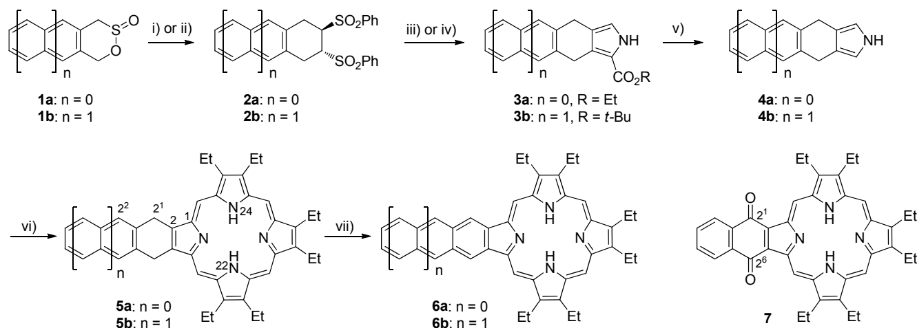
Scheme 1. Reagents, conditions, and yields: i) trans -1,2-bis(phenylsulfonyl)ethylene, toluene, reflux; 89% for 2a ; ii) trans -1,2-bis(phenylsulfonyl)ethylene, o -dichlorobenzene, reflux; 67% for 2b ; iii) CNCH 2 CO 2 Et, t -BuOK, THF, rt; 76% for 3a ; iv) CNCH 2 CO 2 - t -Bu, t -BuOK, THF, rt; 63% for 3b ; v) KOH, (CH 2 OH) 2 , 175 °C; 80% for 4a , 72% for 4b ; vi) tert -butyl 5-(acetoxymethyl)-3,4-diethylpyrrole-2-carboxylate, CH 2 Cl 2 , montmorillonite K-10, rt; TFA, rt; 3,4-diethylpyrrole-2,5-dicarbaldehyde, CH 2 Cl 2 , rt; Et 3 N, DDQ, rt; 25% for 5a , 13% for 5b ; vii) DDQ, toluene, reflux; 75% for 6a , 65% for 6b .
