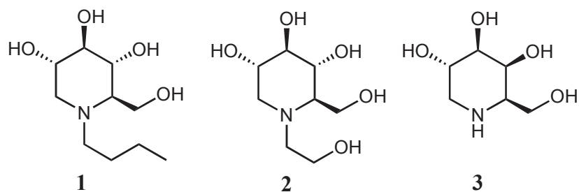
Figure 1. Clinical drugs of iminosugars
