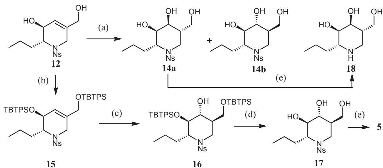
Scheme 3. (a) (1)BH 3 -THF/THF, (2) 3M NaOH/30% H 2 O 2 /37% for 14a /35%, for 14b , (b) TBDPSCl/imidazole/DMAP/ CH 2 Cl 2 /93%, (c) BH 3 -THF/THF, (2) 3M NaOH/30% H 2 O 2 /60%, (d) TBAF/THF/96%, (e) benzenethiol/K 2 CO 3 /MeCN/82%/ for 5 , for 90% for 18
