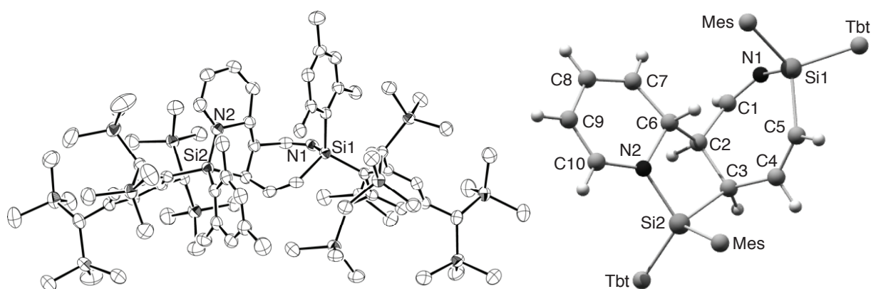
Figure 1. Thermal ellipsoid plot of [ 5 ·hexane] (50% probability) and the ball and stick model of its core structure. In the thermal ellipsoid plot, hydrogen atoms and hexane molecule were omitted for clarity. Selected bond lengths (Å): Si1–N1 1.775(3), Si1–C5 1.886(3), N1–C1 1.210(4), C1–C2 1.546(4), C2–C3 1.537(4), C2–C6 1.544(4), C3–C4 1.512(4), C3–Si2 1.968(3), C4–C5 1.290(4), Si2–N2 1.746(3), N2–C10 1.386(4), N2–C6 1.493(4), C6–C7 1.500(4), C7–C8 1.317(4), C8–C9 1.454(5), C9–C10 1.324(4).
