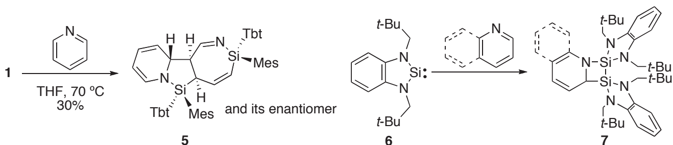
Scheme 3. Reaction of silylene 2 generated from 1 with pyridine and the related reactions.
