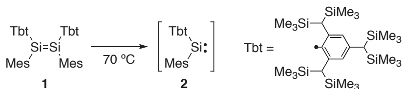
Scheme 1. Thermal dissociation of disilene 1 .
