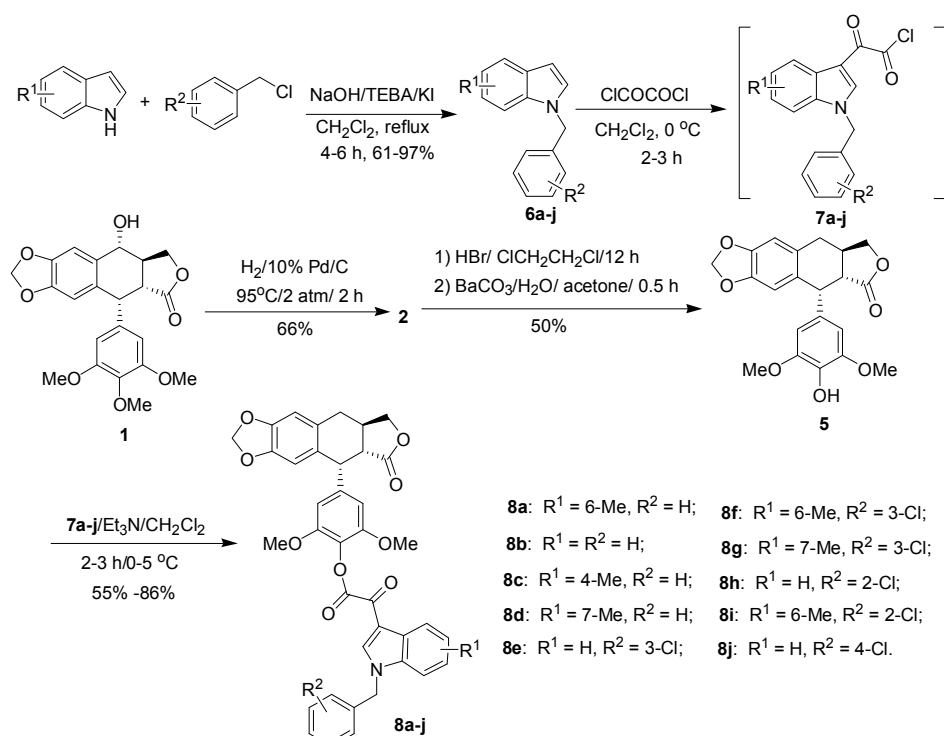
Scheme 1. The synthetic route of O -(deoxypodophyllotoxin-4'-yl)-(N-(un)substituted benzyl)indol-3-ylglyoxylester derivatives ( 8a-j )
