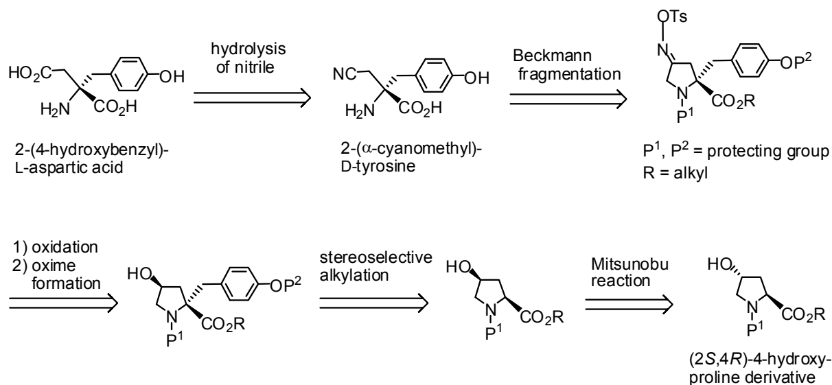
Scheme 1. Retrosynthetic analysis of 2-(4-hydroxybenzyl)-L-aspartic acid and 2-( \alpha -cyanomethyl)-D-tyrosine
