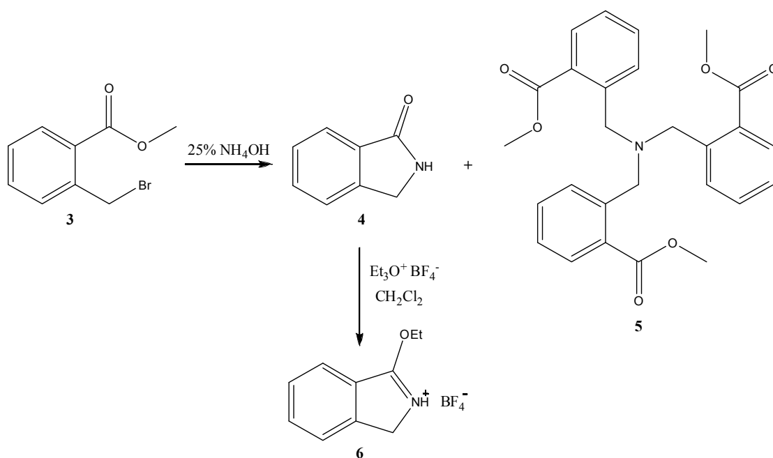
Scheme 2. Synthesis of 1-ethoxyisoindolium tetrafluoroborate 6
