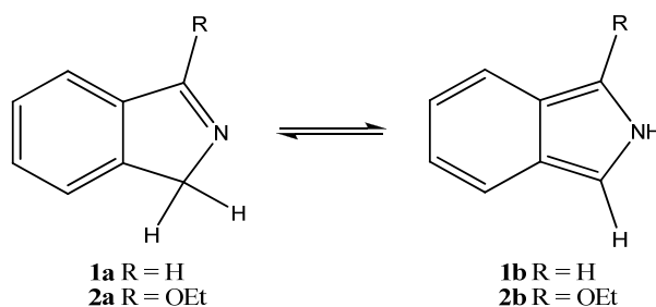
Scheme 1. Tautomerism of unsubstituted isoindole 1 and 1-ethoxyisoindole 2
