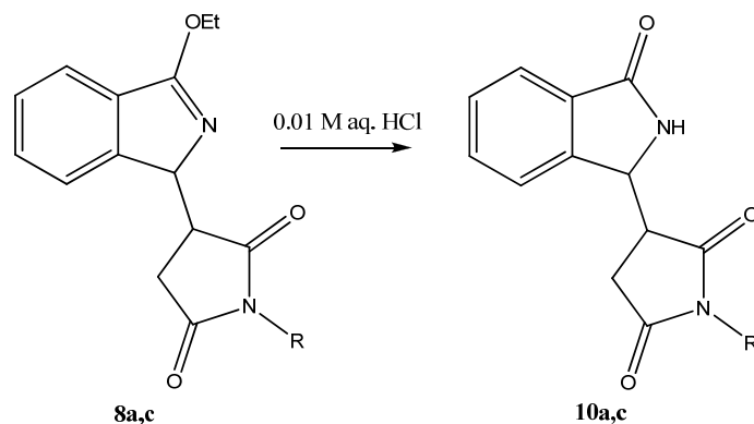
Scheme 4. Hydrolysis of compound 8a,c with the formation of phthalimidine derivatives 10a,c
