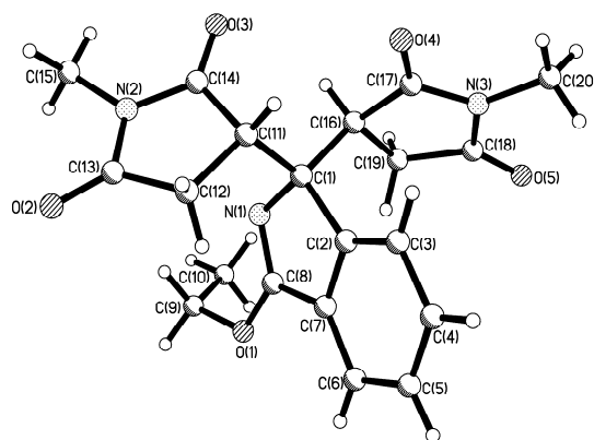
Figure 2. Structure of compound 9b according to X-ray diffraction data
