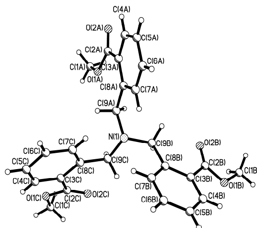
Figure 1. Structure of compound 5 according to X-ray diffraction data
