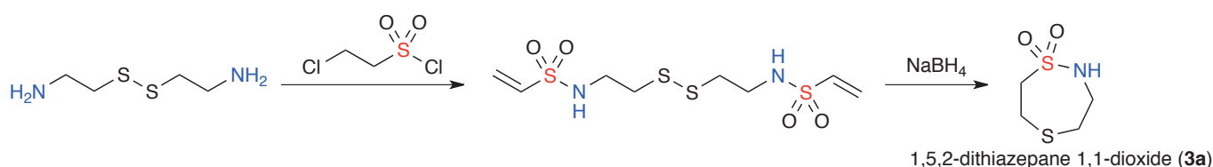
Scheme 2. Reported synthesis of 1,5,2-dithiazepane 1,1-dioxide ( 3a )
