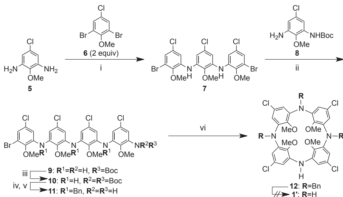
Scheme 1. Attempted synthesis of p -chloroazacalix[4]arene 1' . (i) 5 mol% Pd(OAc) 2 , 7.5 mol% DPEphos, 2.4 equiv t -BuONa, PhMe, 80 °C, 16 h, 53%. (ii) 10 mol% Pd(OAc) 2 , 15 mol% DPEphos, 1.1 equiv t -BuONa, PhMe, 90 °C, 15 h, 68%. (iii) 1.5 equiv Boc 2 O, 0.1 equiv DMAP, THF, reflux, 8 h, 75%. (iv) 3.1 equiv BnBr, 4.0 equiv NaH, DMF, 0 °C to rt, 14 h. (v) TFA, CH 2 Cl 2 , rt, 22 h, 59% in two steps. (vi) 20 mol% Pd(dba) 2 , 30 mol% (±)-BINAP, 2.0 equiv t -BuONa, PhMe, reflux, 18 h, 43%
