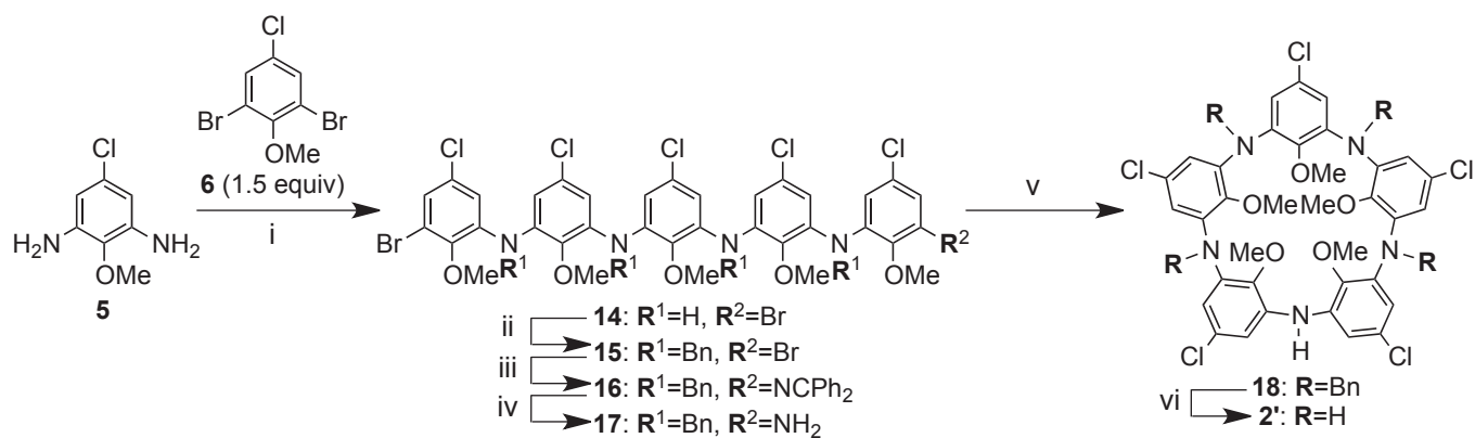
Scheme 2. Synthesis of p -chloroazacalix[5]arene 2' . (i) 10 mol% Pd(OAc) 2 , 15 mol% DPEphos, 2.0 equiv t -BuONa, PhMe, 80 °C, 25 h, 21%. (ii) 6.2 equiv BnBr, 6.9 equiv NaH, DMF, 0 °C to rt, 7 h, 82%. (iii) 1.0 equiv Ph 2 C=NH, 5 mol% Pd(dba) 2 , 15 mol% (±)-BINAP, 2.5 equiv t -BuONa, PhMe, 80 °C, 4 h, 43%. (iv) 1.2 M HCl, THF, rt, 5 h, 98%. (v) 10 mol% Pd(dba) 2 , 30 mol% (±)-BINAP, 2.5 equiv t -BuONa, PhMe, 80 °C, 30 h, 65%. (vi) 4.0 equiv TMSI, CHCl 3 , 50 °C, 23 h, 76%
