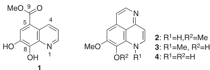
Figure 1. Structures of 1-4
