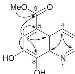
Figure 2. HMBC correlations observed for 1
