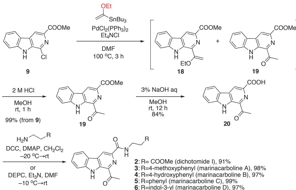
Scheme 4
