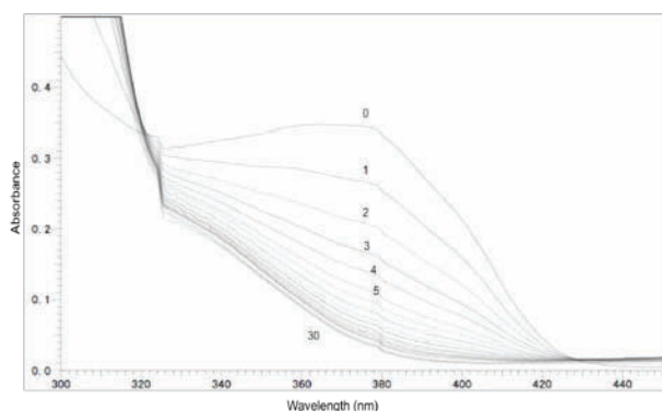
Scheme 4. Photolysis of photoreactive aspartame ( 2 ) in methanol (1 mM) with black light (100W). UV spectra of the photolysis reaction were recorded every 1 min until 15 min, then every 5 min until 30 min.
