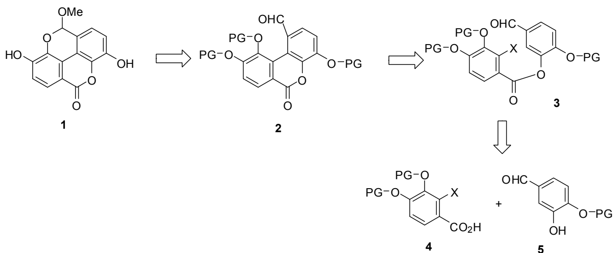
Scheme 1. Retrosynthesis of Nigriganin ( 1 )
