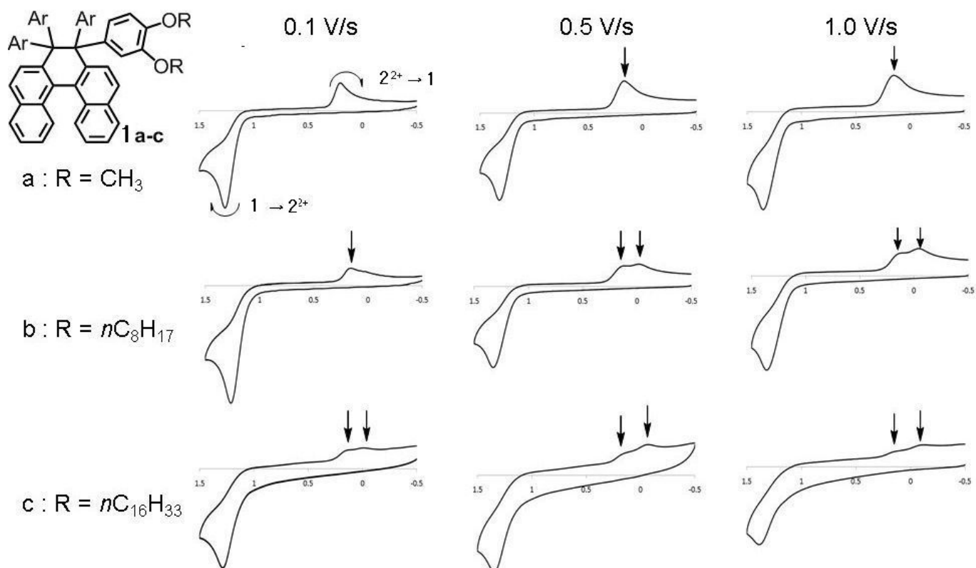
Figure 3. Cyclic voltammograms of 1a-c measured in \text{CH}_2\text{Cl}_2 containing 0.1 M \text{Bu}_4\text{NBF}_4 as a supporting electrolyte ( E/\text{V} vs SCE) at various scan rate at 25 °C. The arrows indicate the top of reduction peaks.
