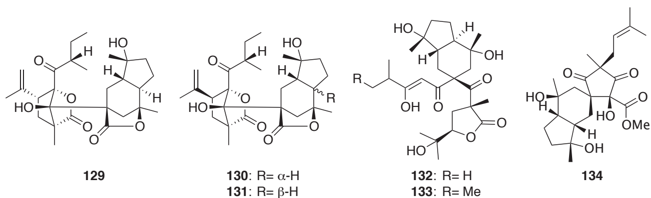
Figure 14. Meroterpenoids ( 129–134 ) from Hypericum plants
