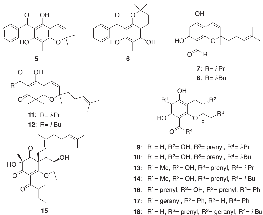
Figure 2. PAPs with bicyclic structures ( 5–18 ) from Hypericum plants
