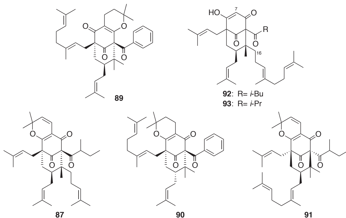
Figure 8. PPAPs with bicyclo[3.3.1]nonane-2,4,9-trione core ( 89–93 ) from Hypericum plants
