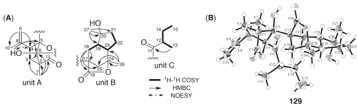
Figure 15. (A) Selected 2D NMR correlations and (B) ORTEP drawing of biyoulactone A ( 129 )
