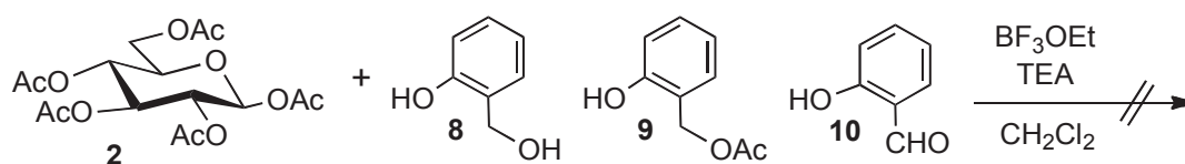
Scheme 2. Glucosidation of \beta -pentaacetylglucose 2 with salicyl derivatives 8–10
