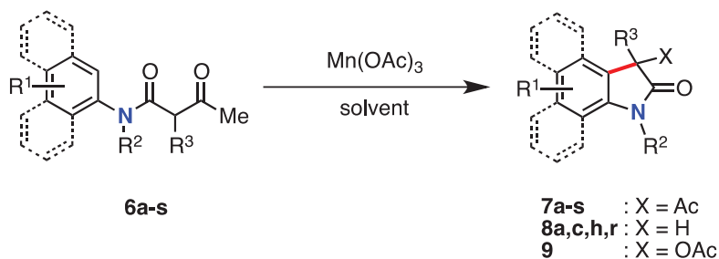
Scheme 3. Oxidation of N ,2-Dialkyl- N -aryl-3-oxobutanamides 6a-s with \text{Mn}(\text{OAc})_3
