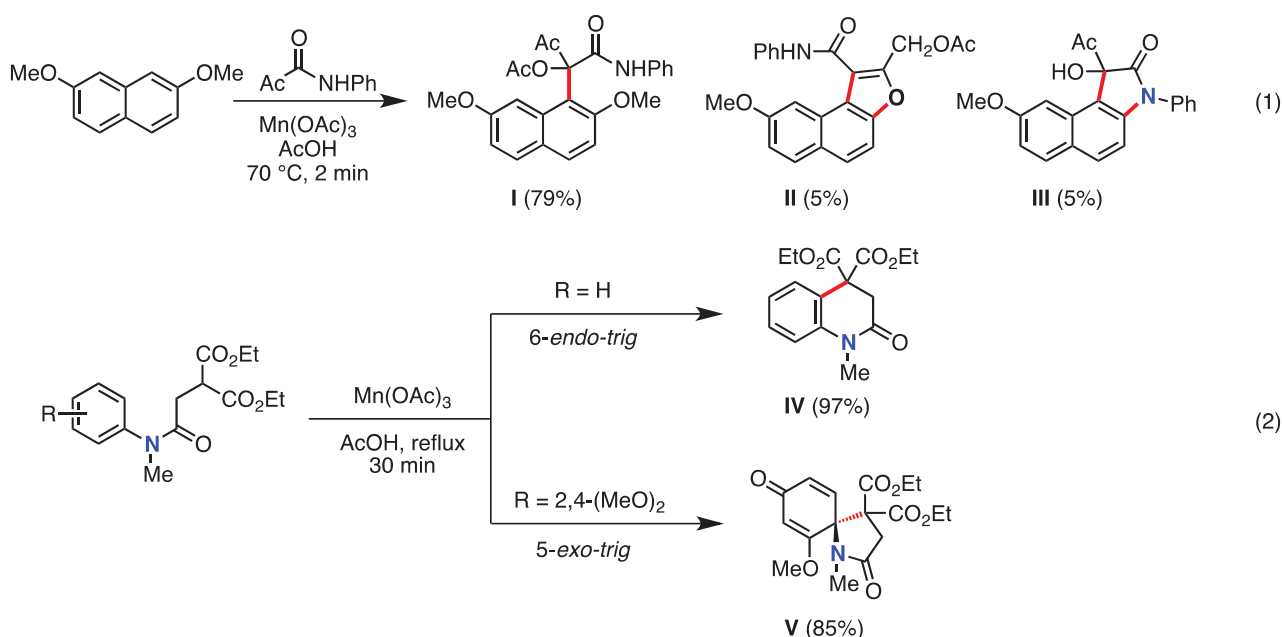
Scheme 1. Carbon-Carbon Bond Formation Using Mn(III)-Based Oxidation
