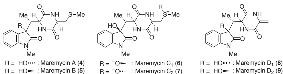
Figure 2. Structures of maremycins
