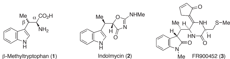
Figure 1. β-Methyltryptophan and related natural products
