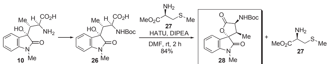
Scheme 9. Attempt to prepare amino acid 24
