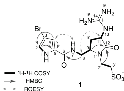
Figure 1. Selected 2D NMR correlations for 2-debromonagelamide U ( 1 )
