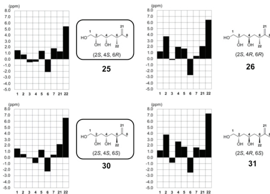
Figure 3. Difference in 13 C NMR chemical shifts between amphidinin A ( 1 ) 2 and synthetic C1-C8 segment diastereomers ( 25 , 26 , 30 , and 31 )(C 6 D 6 , 150 MHz)
