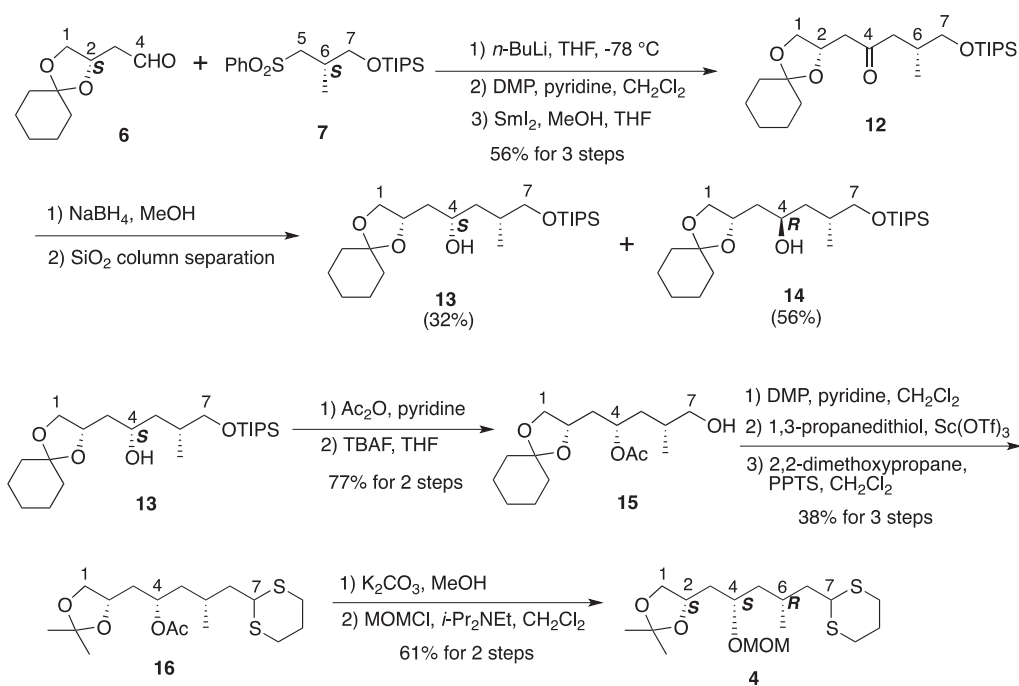
Scheme 2. Synthesis of the C-1-C-7 segment 4 from 6 and 7
