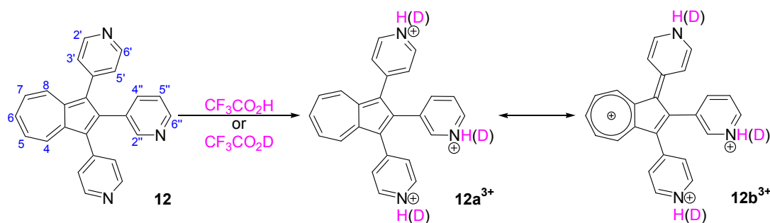
Scheme 4. Protonation of 12 in \text{CF}_3\text{CO}_2\text{H} (or \text{CF}_3\text{CO}_2\text{D} )
