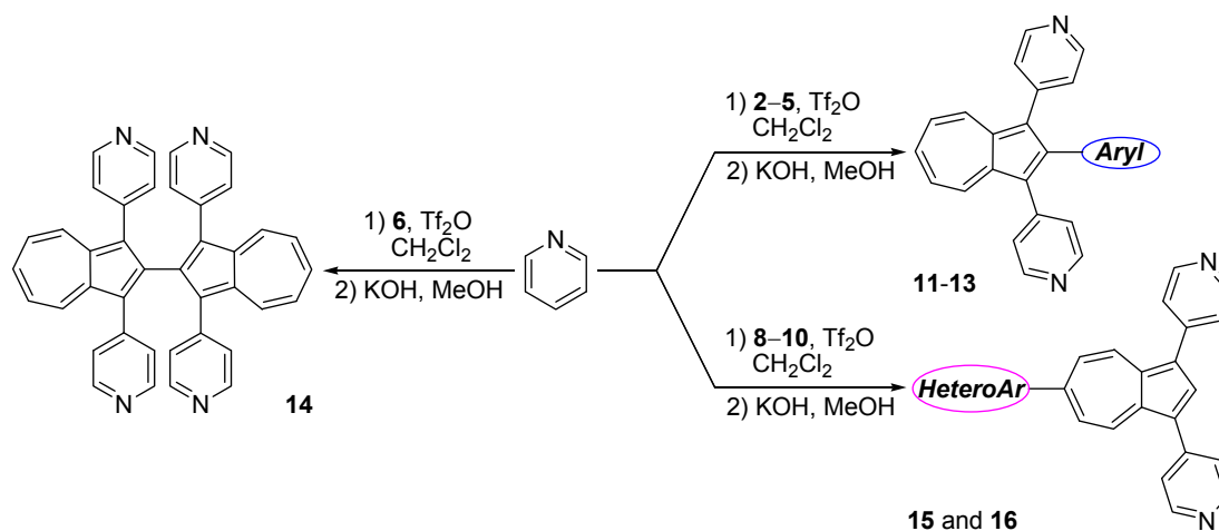
Scheme 3. Reaction of 2-aryl- and 6-heteroarylazulenes with TPT
