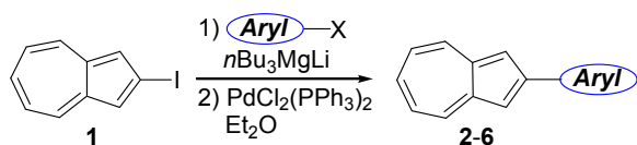
Scheme 1. Palladium-catalyzed cross-coupling reaction of 1 with arylmagnesate reagents
