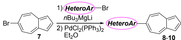
Scheme 2. Palladium-catalyzed cross-coupling reaction of 7 with heteroarylmagnesate reagents
