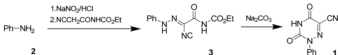
Scheme 1. Synthesis of starting 1,2,4-triazine ( 1 )
