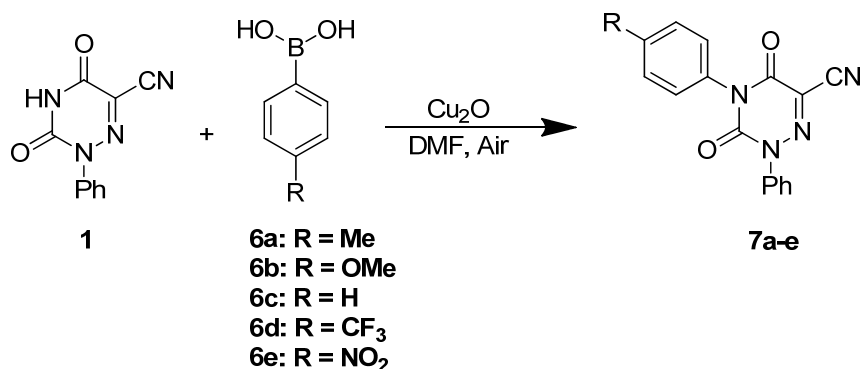
Scheme 4. Chan-Lam coupling
