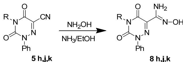
Scheme 5. Addition of hydroxylamine to the nitrile group
