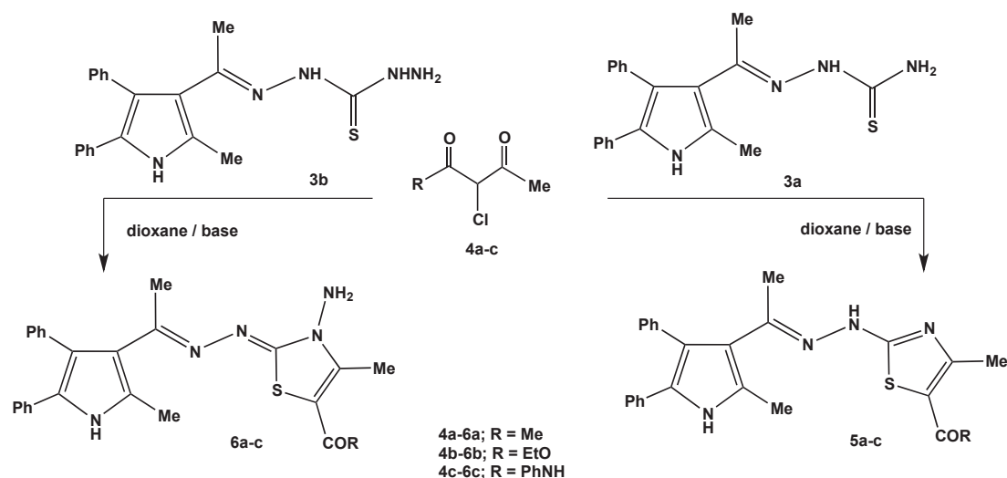
Scheme 2. Synthesis of compounds 5a-c and 6a-c
