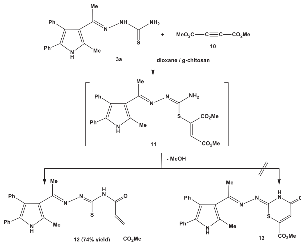
Scheme 4. Synthesis of compound 12
