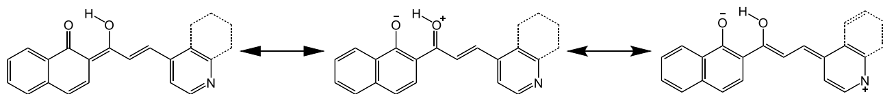
Scheme 2. Resonance structures of cis -keto form of 3 and 4
