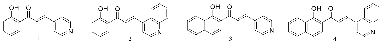
Figure 2. Structure of 2HC derivatives examined in this work
