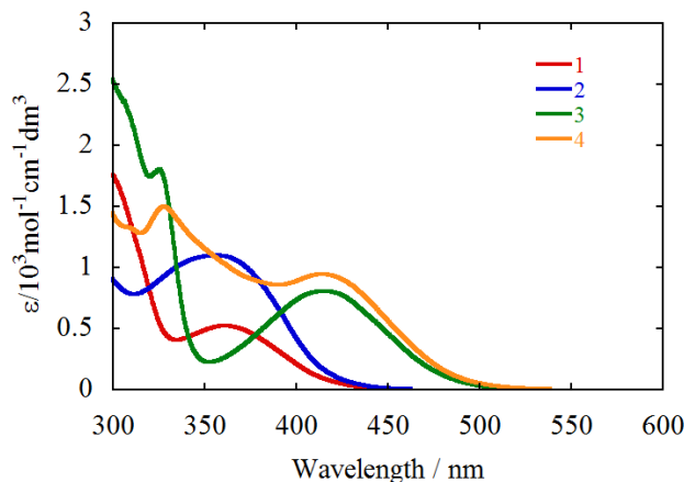
Figure 3. Absorption spectra of 1-4 in benzene
