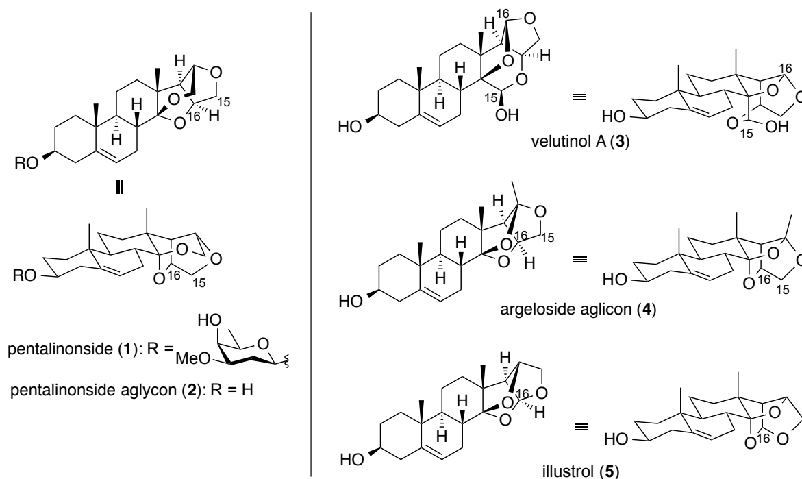
Figure 1. Structures of seco -pregnanes with cage-like DEF-rings
