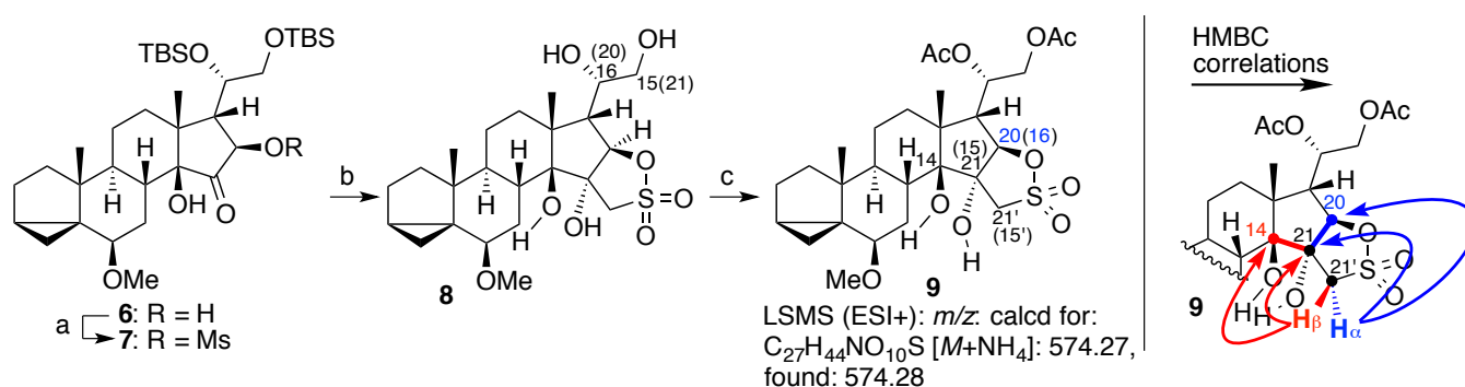
Scheme 2. Unsuccessful route for F-ring formation. Reagents and conditions: a) MsCl, pyridine, rt, 2.5 h, 88%; b) n\text{Bu}_4\text{NF} , THF, rt, 12 h, 45%; c) pyridine, \text{Ac}_2\text{O} , 86%. Ms = methanesulfonyl
