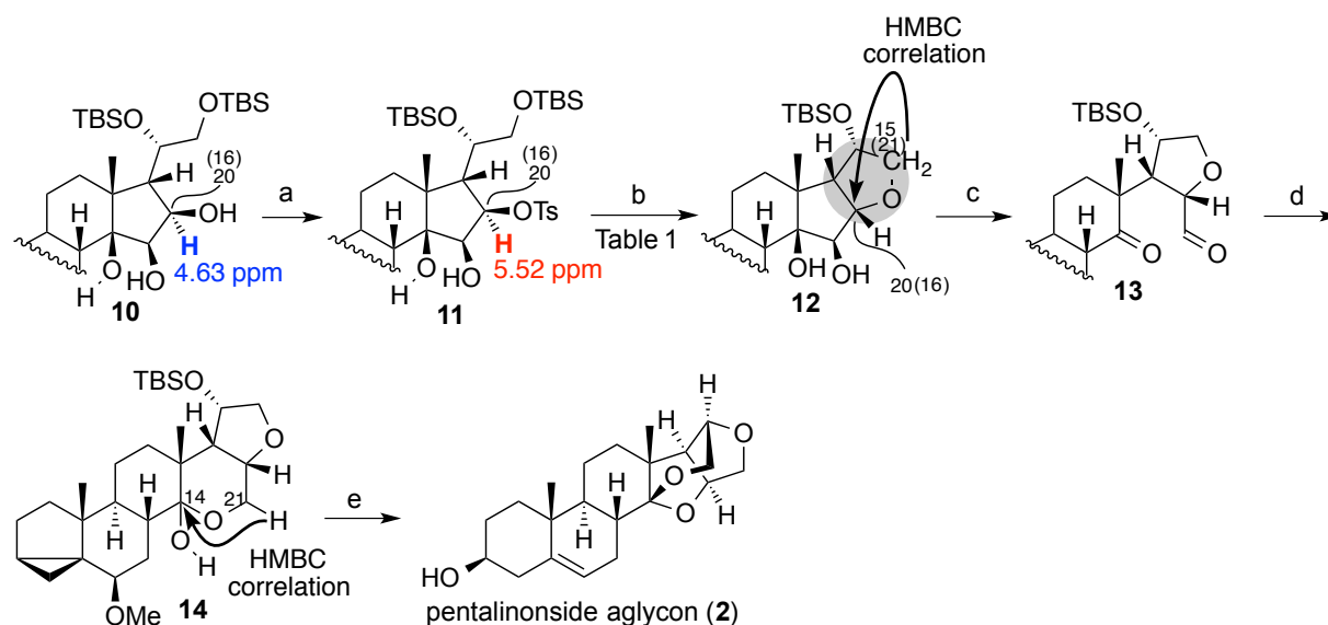
Scheme 3. Synthesis of the pentalinonside aglycon ( 2 ). Reagents and conditions: a) TsCl, DMAP, CH 2 Cl 2 , rt, 2 h, 93%; b) n Bu 4 NF/AcOH (1:2), THF, reflux, 2 h, 62%, for yields and conditions see Table 1; c) NaIO 4 , THF/H 2 O (1:1), rt, 5 h, 81%; d) NaBH 4 , MeOH, 0 °C, 10 min, 71%; e) HClO 4 , 1,4-dioxane/H 2 O (5:4), rt, 2 h, 95%. Ts = p -toluenesulfonyl, DMAP = 4-dimethylaminopyridine
