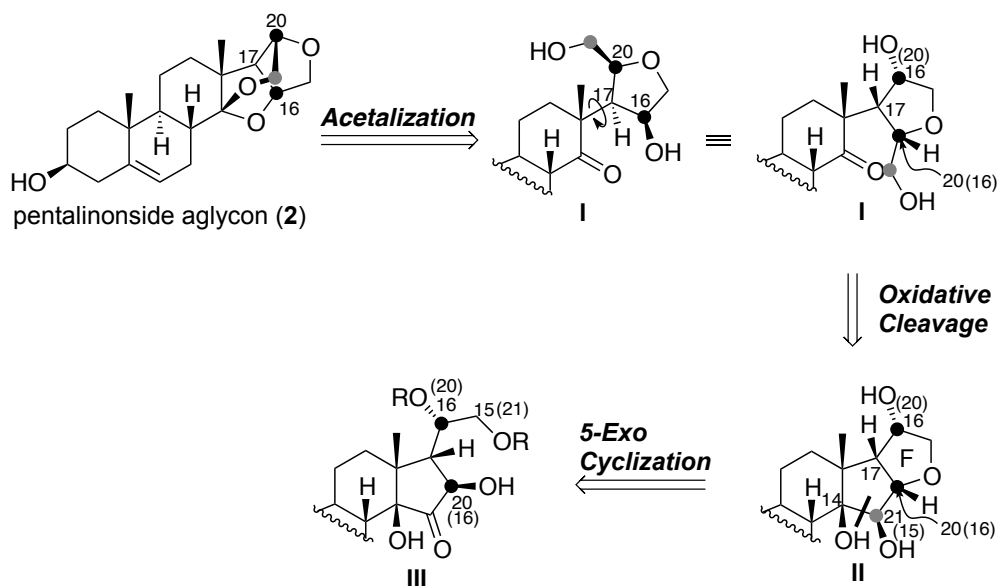
Scheme 1. Retrosynthetic analysis
