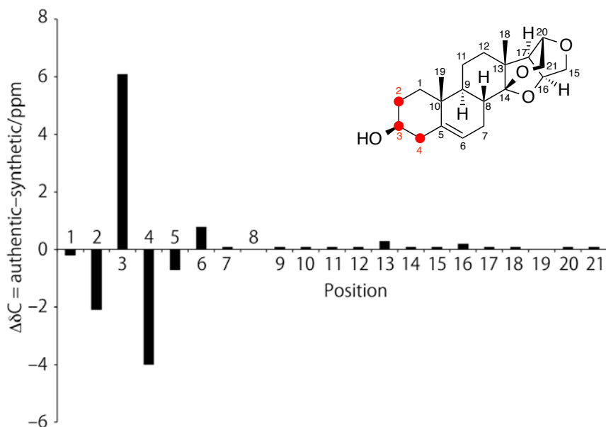
Figure 3. \Delta\delta C values of the authentic pentalinonside aglycon and synthetic aglycon
