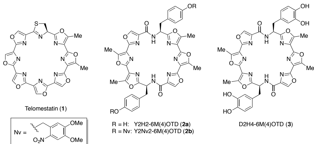
Figure 1. Chemical structures of telomestatin (1) and 6OTDs (2a, 2b and 3)
