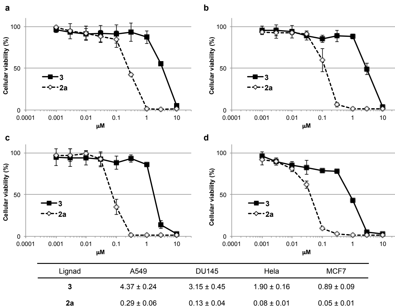
Figure 2. Dose-response curves of 3 and 2a for growth inhibition of A549 (a), DU145 (b), HeLa (c) and MCF7 (d) cells 6 days after drug treatment. The IC_{50} values (μM) are the mean ± SD of triplicate assays.
