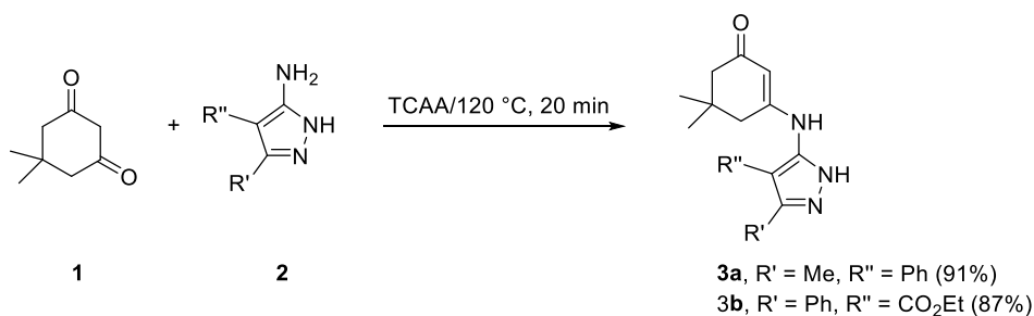
Scheme 1. Synthesis of enamines 3a,b
