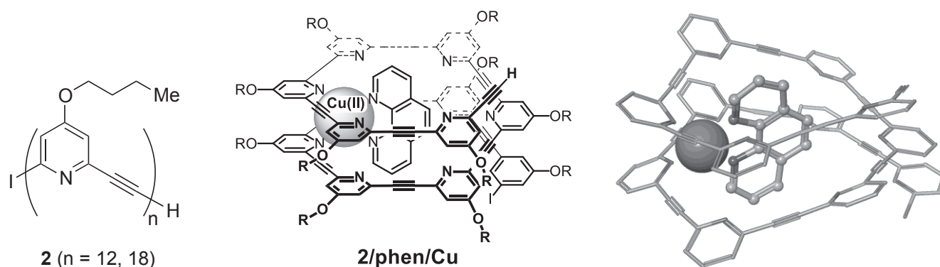
Figure 2. (left) meta -Ethylnylpyridine oligomer 2 . (center and right) Schematic illustrations of helical complex 2 /phen/Cu, cross-linked from inside the helix by Cu(II) and phenanthroline, showing a chiral memory effect (ref 15).
