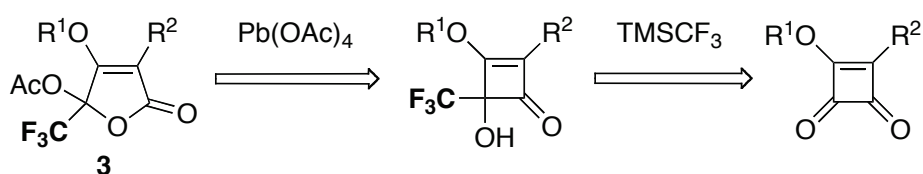
Scheme 2. New method for the synthesis of \gamma -trifluoromethylated tetronates 3 from squarates
