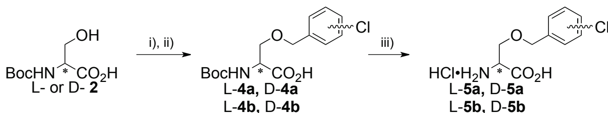
Scheme 2. Synthesis of O -benzylserine derivatives 5a and 5b
