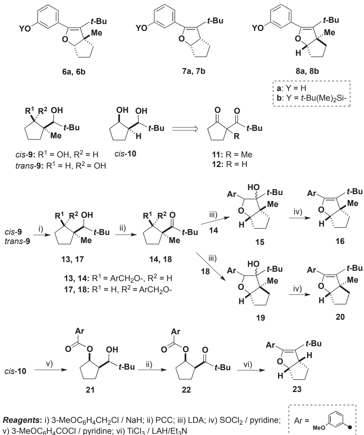
Scheme 1. Synthesis of bicyclic dihydrofurans bearing a 3-siloxyphenyl group
