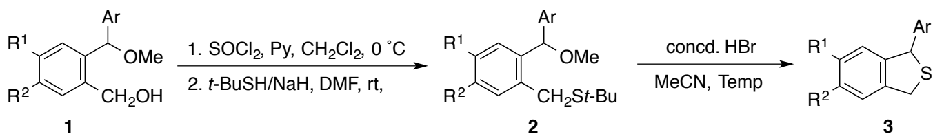
Scheme 1
