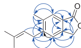
Figure 2. Key HMBC ( \curvearrowright ) correlations of 1
