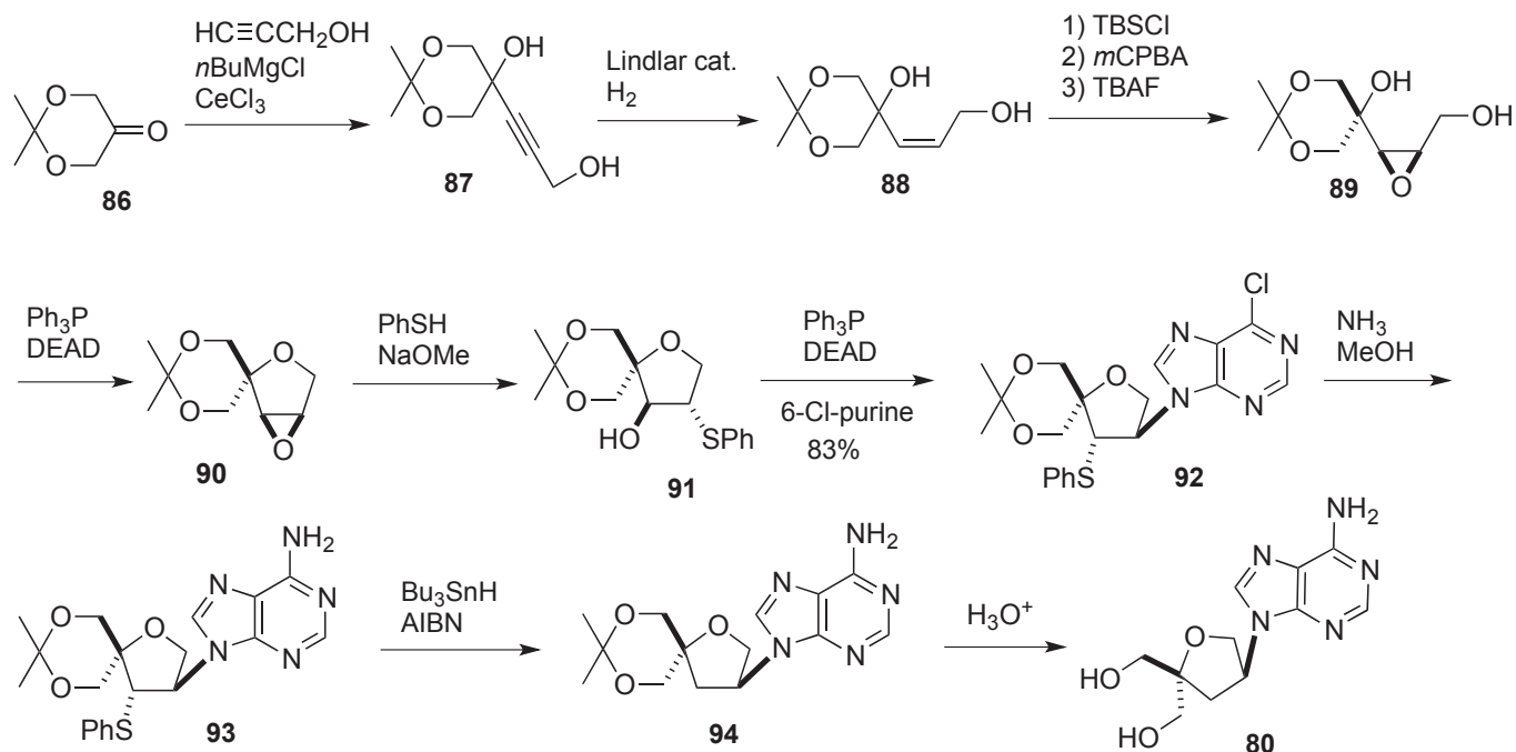
Scheme 11. Synthesis of 4'-hydroxymethyl-iso-ddA
