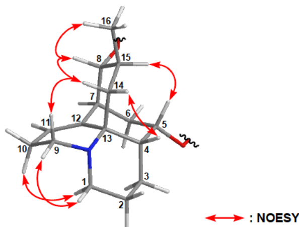
Figure 2. Selected NOESY correlations for phlendumine A ( 1 )
