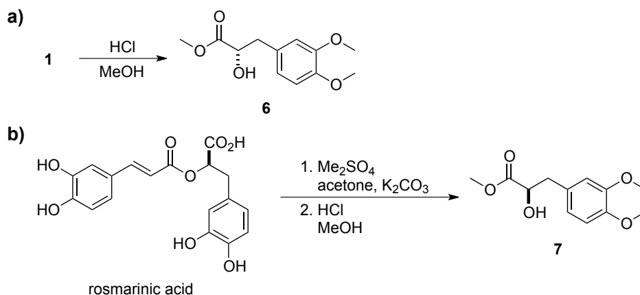
Scheme 2. Chemical derivatizations of (a) phlendumine A ( 1 ) to 6 and (b) rosmarinic acid to 7
