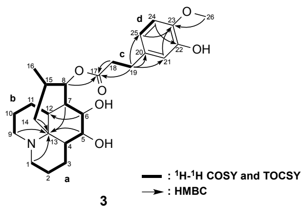
Figure 5. Selected 2D NMR correlations for phlenumidine C ( 3 )
