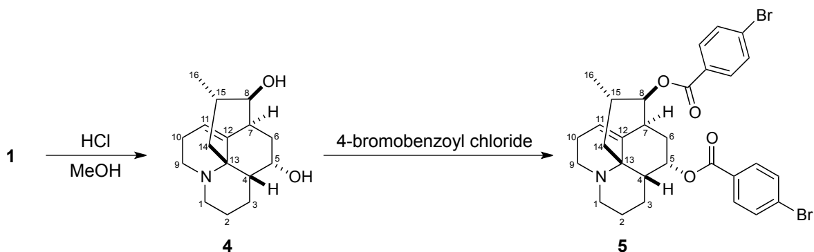
Scheme 1. Chemical derivatization of phlendumine A ( 1 ) to 4 and 5
