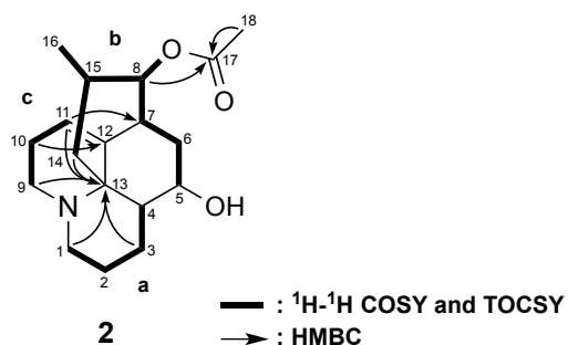
Figure 3. Selected 2D NMR correlations for phlendumine B ( 2 )
