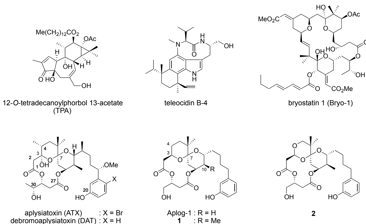
Figure 1. Structures of PKC activators
