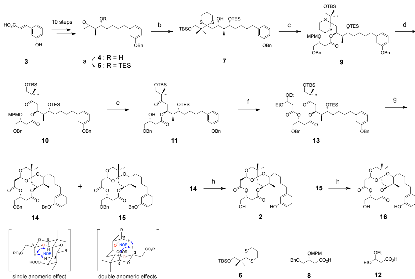
Scheme 1. Synthesis of 2 , (a) TES-Cl, imidazole, THF, 89%. (b) 6 , n -BuLi, THF, 84%. (c) 8 , DCC, DMAP, CH 2 Cl 2 , 57%. (d) I 2 , NaHCO 3 , MeCN, 63%. (e) DDQ, CH 2 Cl 2 , H 2 O, 83%. (f) 12 , TCB-Cl, Et 3 N, DMAP, toluene, 90%. (g) TMSOTf, CH 2 Cl 2 , 14 : 10%, 15 : 14%. (h) H 2 , 10% Pd/C, EtOH, 2 : 78%, 16 : 83%.
